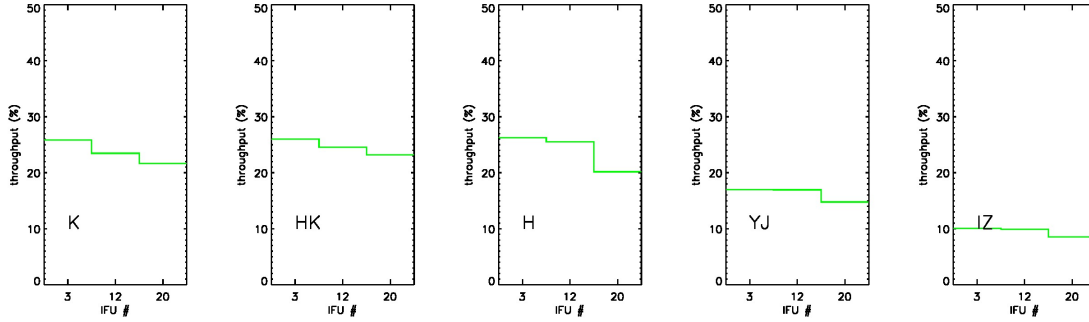
Figure 23: Total instrument transmission for the three detectors and all five bands.
