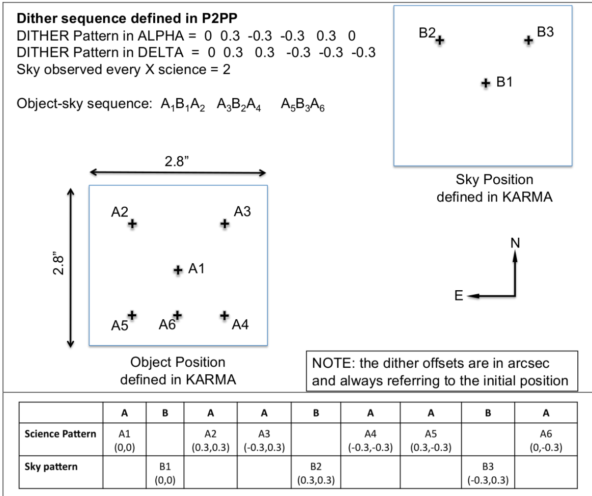
Figure 15: An illustration of the dither pattern that can be constructed with the free-dither template in P2PP. The sequence for just 1 IFU is shown, since it will be identical for all of them. This example is for 6 object frames and sky frequency = 2, which gives in total 3 sky frames in the sequence ABA ABA ABA.
