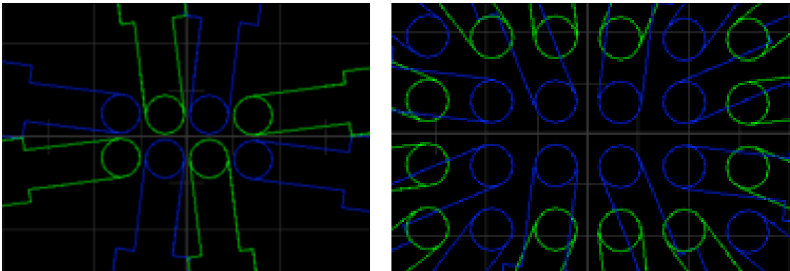
Figure 21: Positions of arms during observations with template KMOS_spec_obs_mapping8 (left side) and KMOS_spec_obs_mapping24 (right side).
