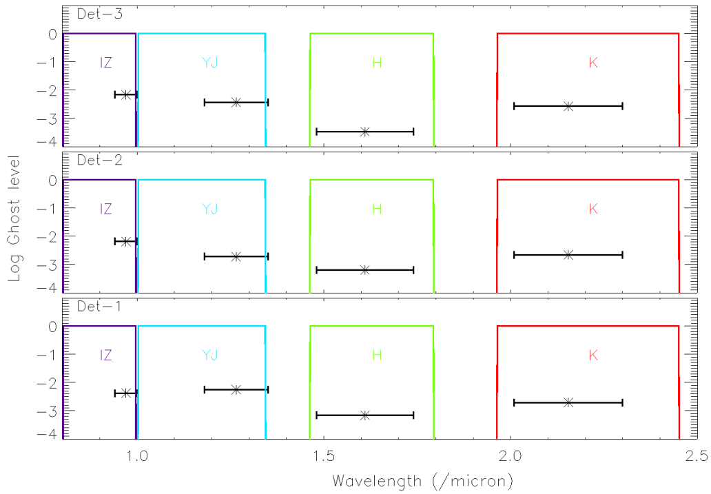
Figure 18: Ghost level as a function of wavelength, for all three detectors. The ghost level is defined as the intensity of the ghost image divided by the intensity of the source that has generated it. The coloured boxes identify the full wavelength coverage in each band (IZ, YJ, H, K). The horizontal error bars denote the fraction of the band affected by the ghost. It can be noted that the level is less than 1 part in 100 and only affects a fraction of the wavelengths, especially in the IZ and YJ bands. The ghost is not present in the HK band.
