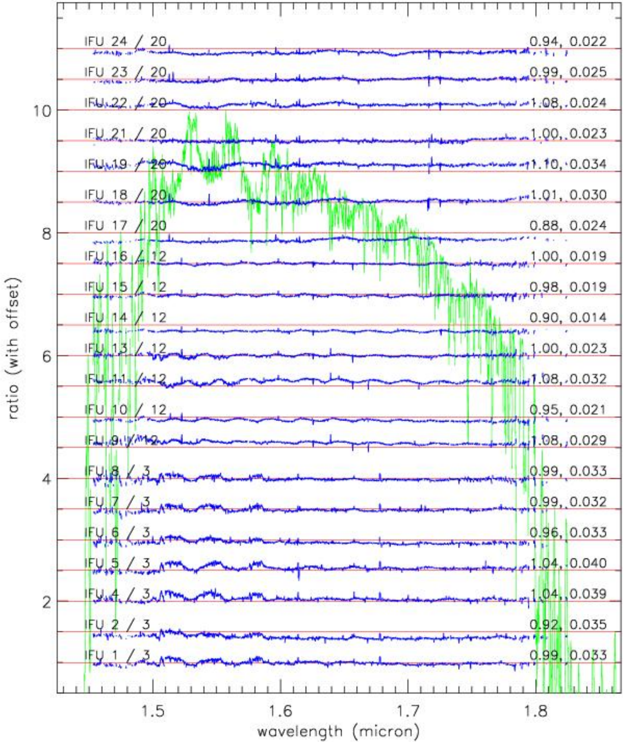
Figure 16: Comparison between the measurements of the 3-arm standard star template and all 24-arms sciencepattern standard star template (Davies et al. 2013, A&A, 558, A56). In the 3-arm standard star the IFUs used are number 3,12 and 20 (one per each spectrograph). The green curve in the background shows the extracted spectrum for a standard star in the H-band. The overplotted blue curves are the ratio (in arbitrary scales and offsetted) between the spectra in each IFU respect to those taken in just 3 reference arms (3,12,20) taken via the 3- arm standard star template, as labelled on the left hand side. For each IFU on the right the mean ratio and the standard deviation are indicated (for regions where the signal-to-noise is above a minimum threshold). This suggests that using just 3 arms to calibrate all IFUs is sufficient at the level of precision of a few percent.
