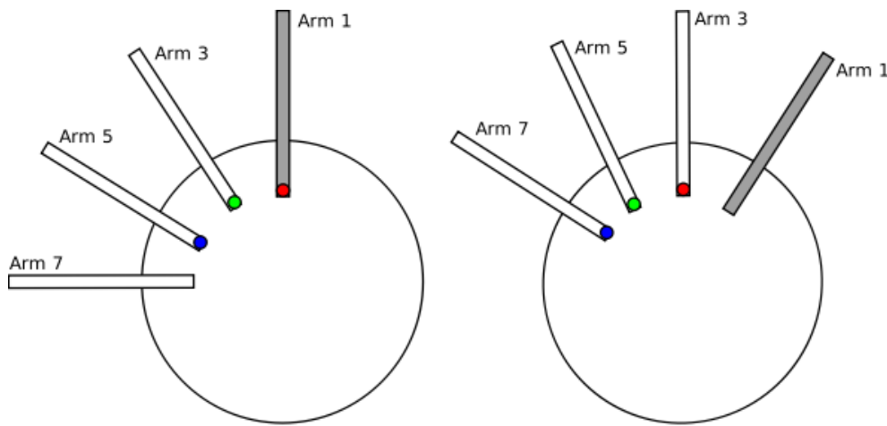
Figure 22: The idea behind the rotator optimisation: Let Arm 1 be locked e.g. after a hardware failure. Left: In the original configuration given by the KARMA set up file the red target cannot be observed. Right: After rotating the instrument and recalculating the mapping between targets and arms all targets are observable. An optimisation like this might be of special interest if the red target has higher priority than the others.
