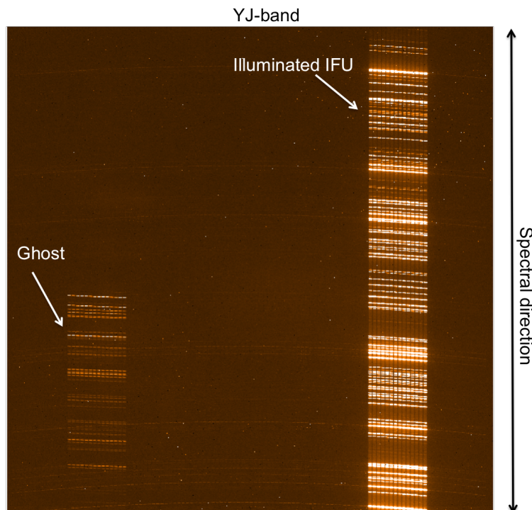
Figure 17: Image in the YJ-band, with one single IFU illuminated with a Argon+Neon calibration lamp (on the right). The ghost is visible on the left side of the array. The colour scale has been enhanced to show the ghost, since the level of the ghost is less than 1% for all bands.
