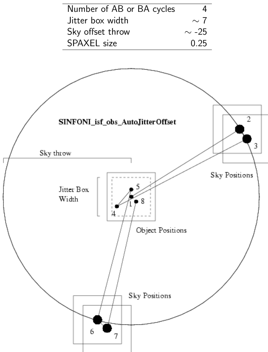
Figure 18: An illustration of the offset sequence taken with the AutoJitterOffset template (“Number of exposure per Offset” = 1). The large circles for the sky position indicate that these observations are performed in open loop.
