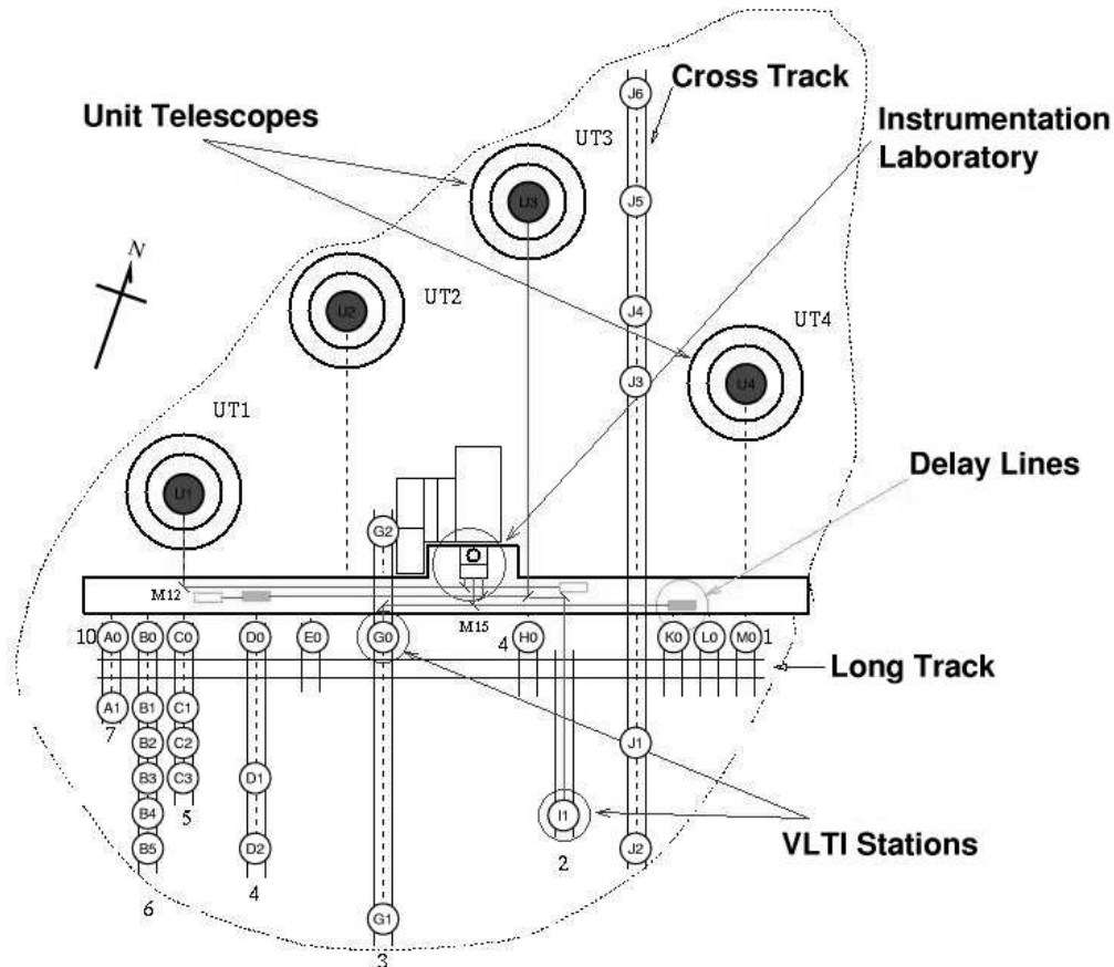
Figure 6: Layout of VLTI telescope locations.
