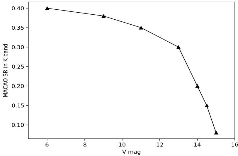
Figure 5: MACAO Strehl ratio (SR) in K-band as a function of V magnitude.
