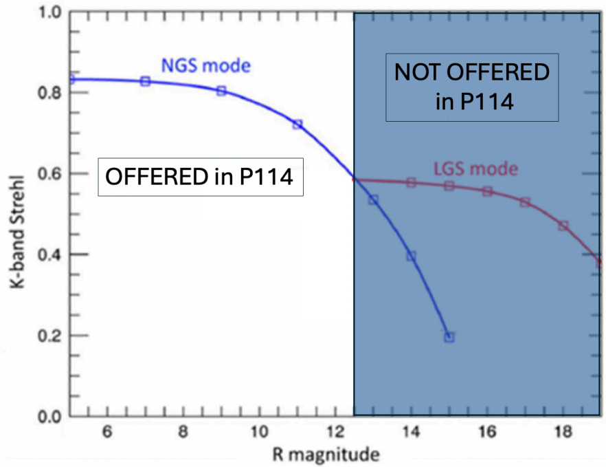
Figure 5: Expected Strehl ratio (SR) in K-band of NGS-VIS (from P114) and LGS-VIS (from P117) modes.
