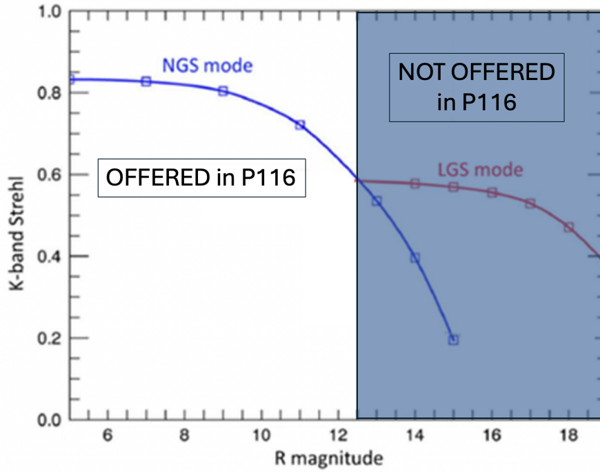
Figure 6: Expected Strehl ratio (SR) in K-band of NGS-VIS in P116 and LGS-VIS (foreseen for P117) modes.
