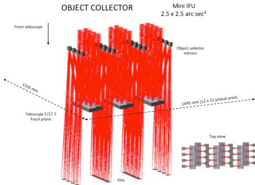
Figure 8: The pick object configuration. Focal plane is filled with stripes of patrol mirrors and the object selector mirrors select a 2.5x2.5 arcseconds area within a pickup area (12x12 arcsecond in this figure).
