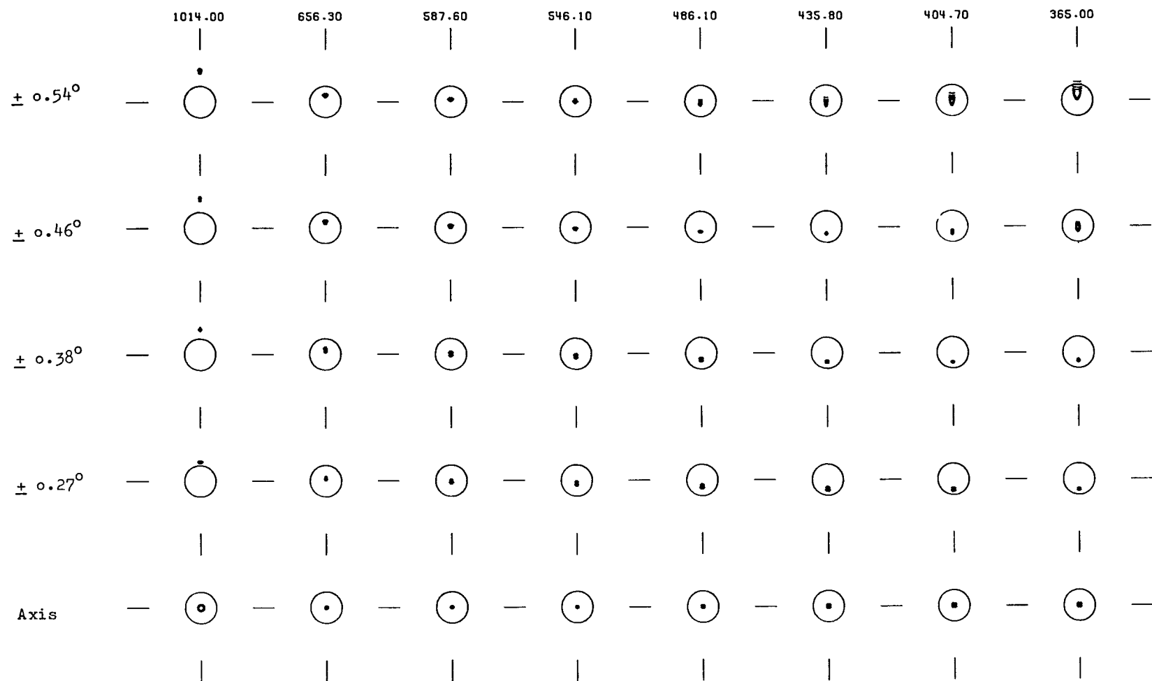
Fig. 10 2.2 m telescope for MPI with strict R-C mirror constants and doublet corrector of two different glasses (PK 50 and BaF 3). Field \pm 0.54^\circ . Spot diagrams. (Circle = 0.48 arcsec = 40 \mu )
