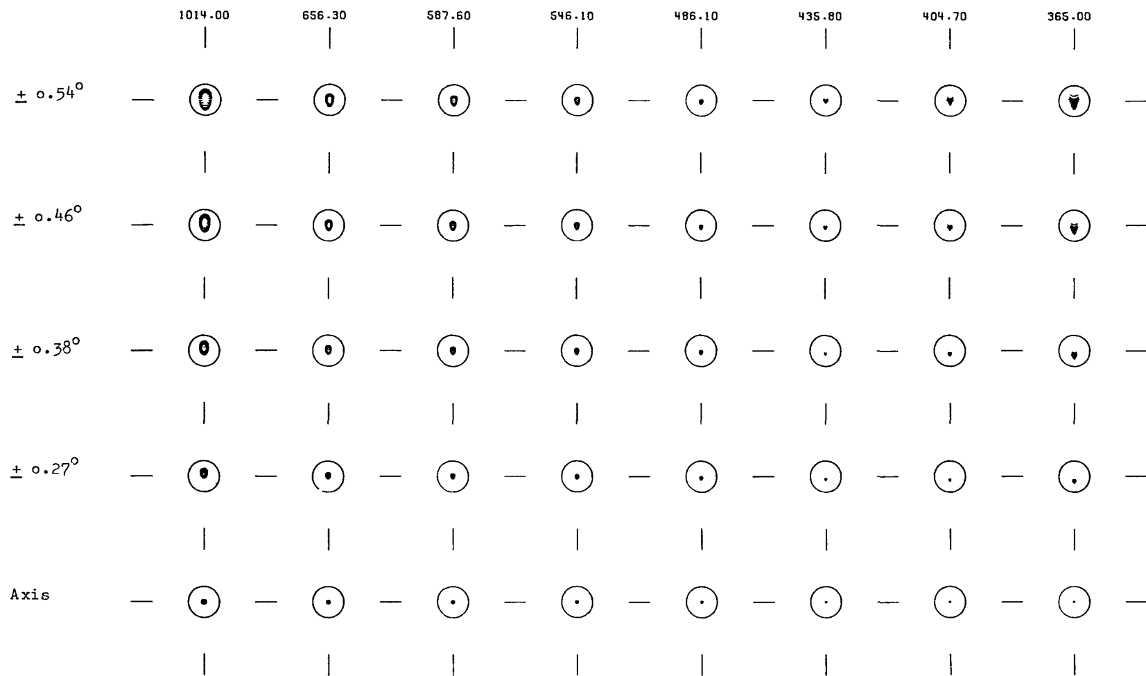
Fig. 9 2.2 m telescope with quasi R-C mirror constants and doublet corrector of one material. Optimized for blue. Field \pm 0.54^\circ . Spot diagrams. (Circle = 0.47 arcsec = 40\mu )
