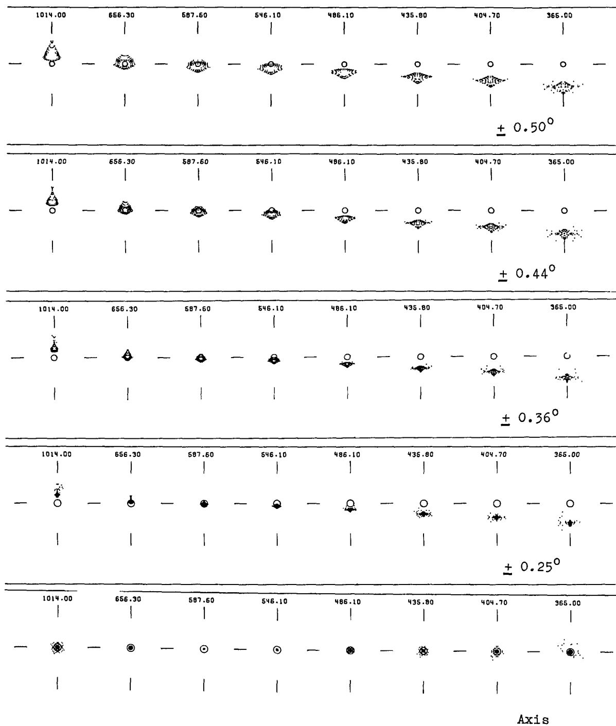
Fig. 24 Focal reducer for 3.5 m telescope. Field lens and Schmidt camera with shifted pupil. Spot diagrams. (Circle = 0.50 arcsec = 14/μ) Reduction f/8 to f/1.7. Image radius = 1221 mm.
