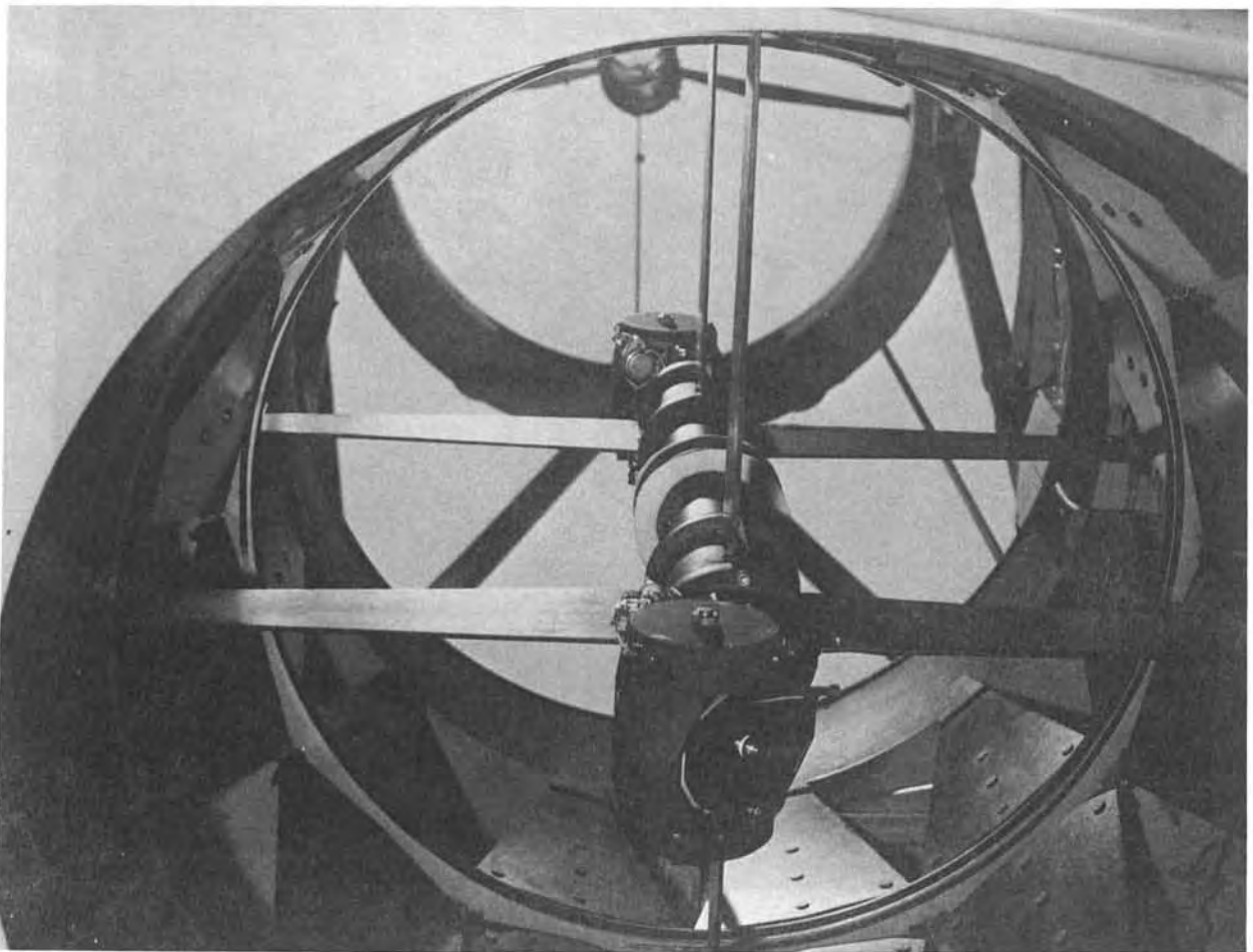
Fig. 4 Photo of the first turret of flat mirrors. The turret of secondary mirrors can be seen reflected in the primary.
