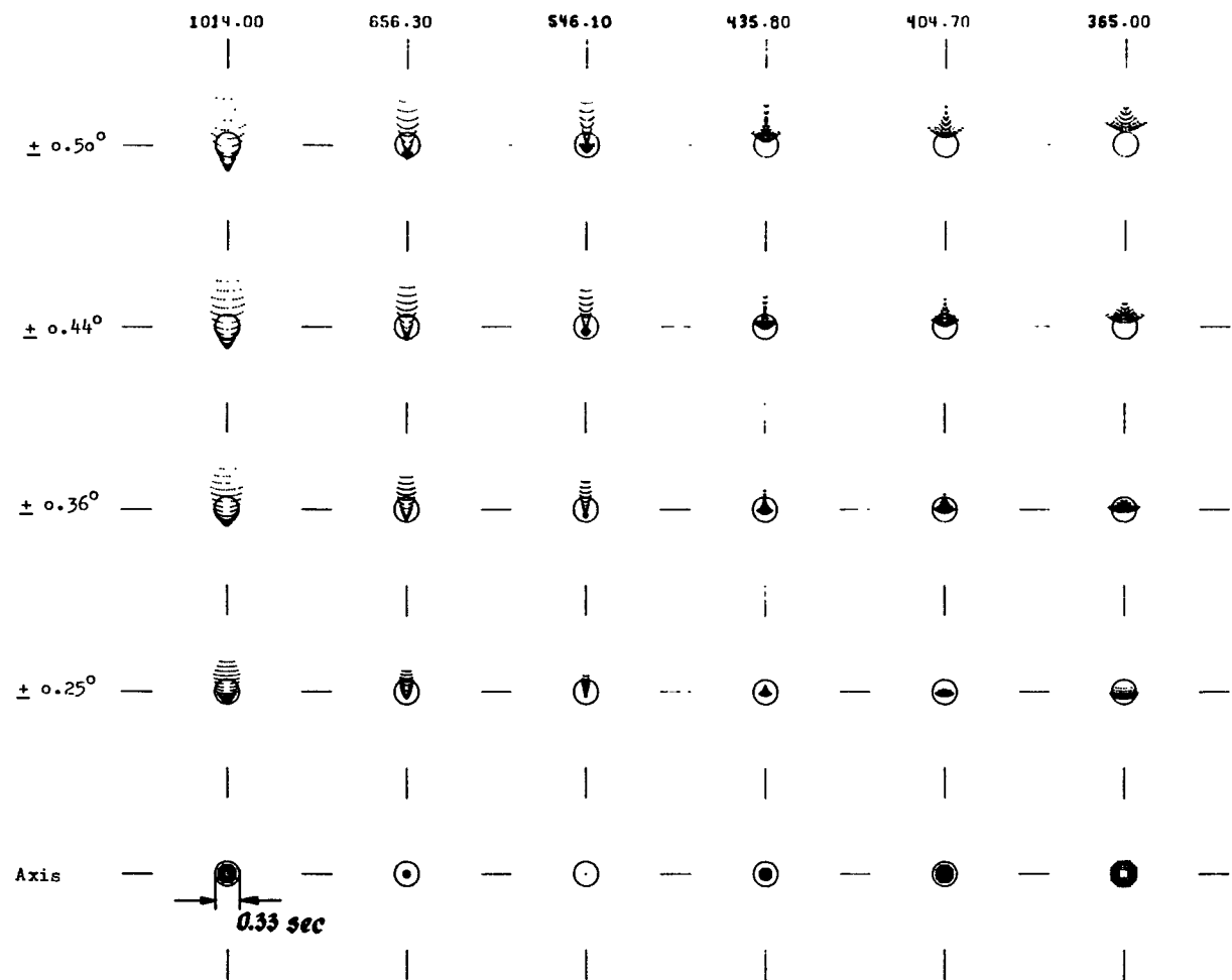
Fig. 4 1.52 m telescope with strict R-C mirror constants and doublet corrector of one material. Field \pm 0.5^\circ . Best focus for 546 nm. Spot diagrams. (Circle = 0.33 arcsec = 20/\mu )
