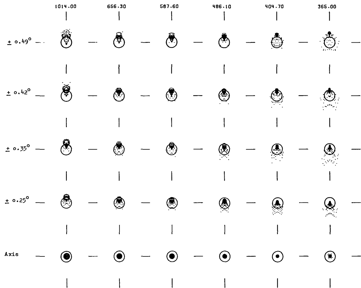
Fig. 17 3.5 m telescope for ESO with modified plate corrector for primary focus as shown in Fig. 16. Field \pm 0.49^\circ (no vignetting). Spot diagrams. (Circle = 0.50 arcsec = 25/\mu )
