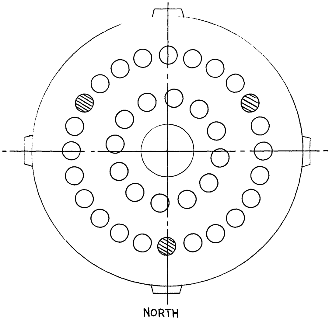
Fig. 4 Position in defining points in primary mirror cell.
