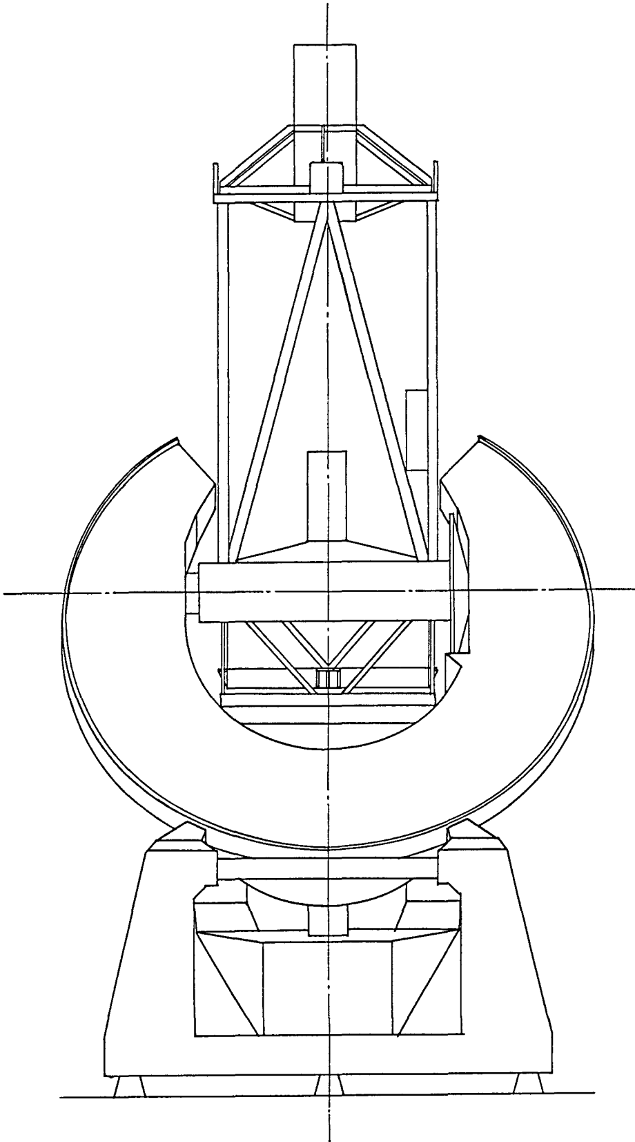
Fig. 2 Anglo-Australian 150-inch telescope.
