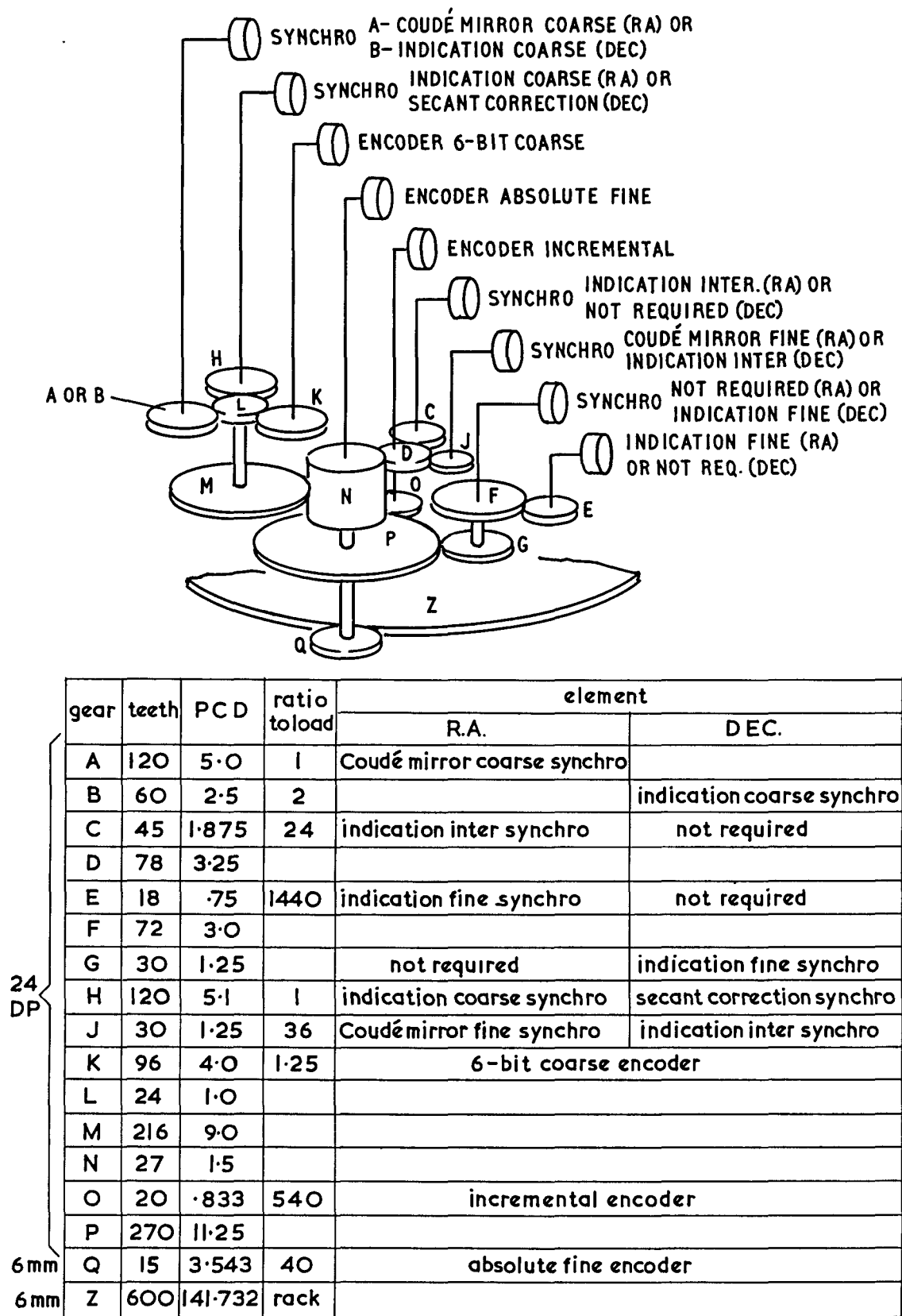
Fig. 2 Schematic layout of encoder drives.
