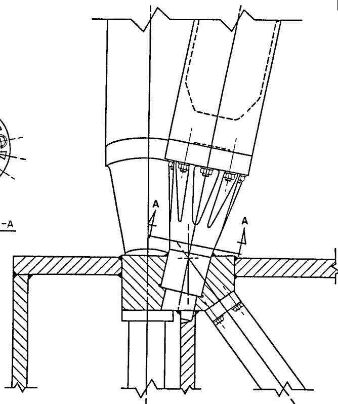
Fig. 5 Serrurier connection.
