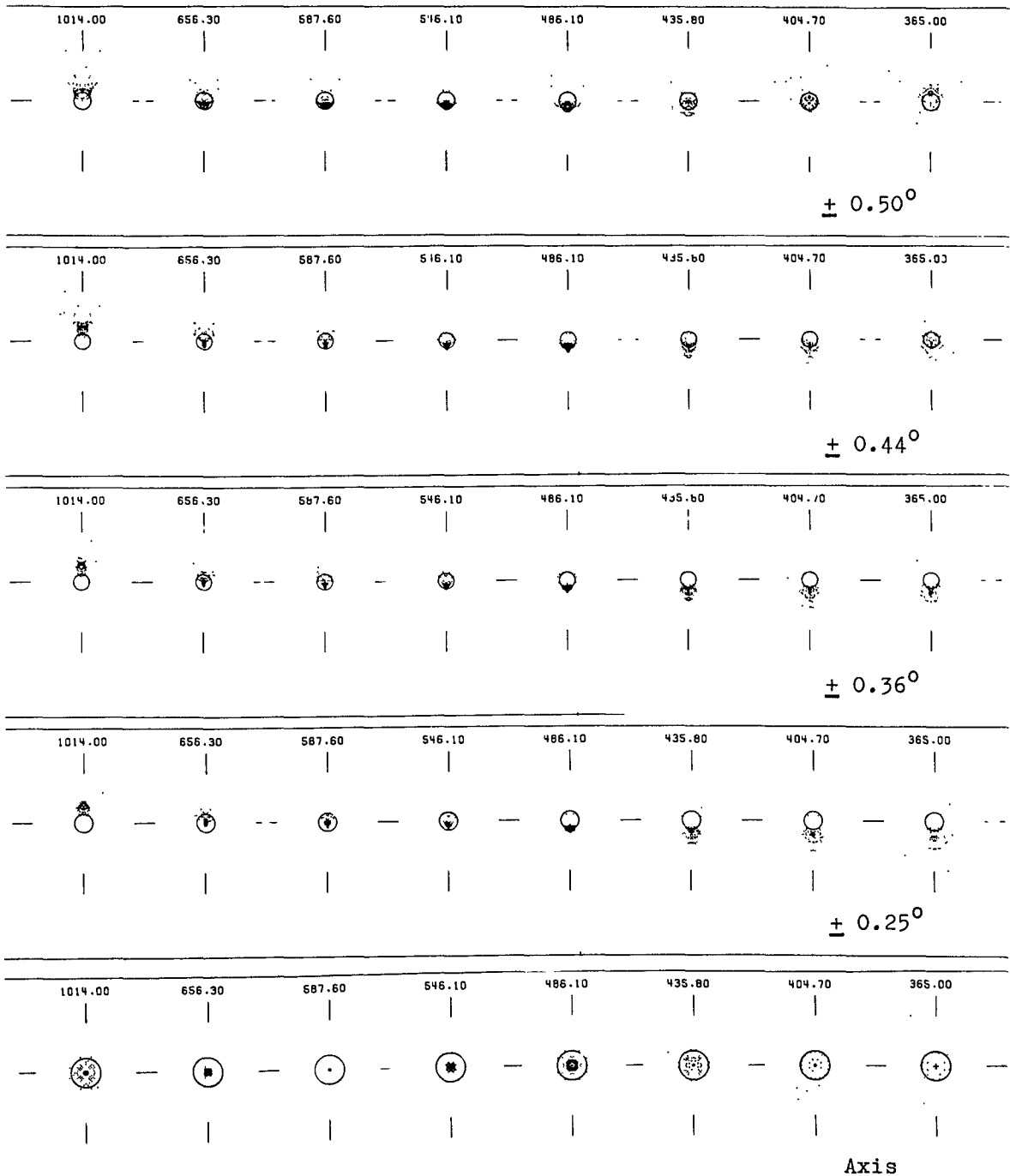
Fig. 25 Focal reducer for 3.5 m telescope. Doublet corrector ( uncorrected intermediate image), field lens and Schmidt camera with shifted pupil. Spot diagrams. (Circle = 0.50 arcsec = 14/ \mu ) Reduction f/8 to f/1.7 . Image radius = 1060 mm.
