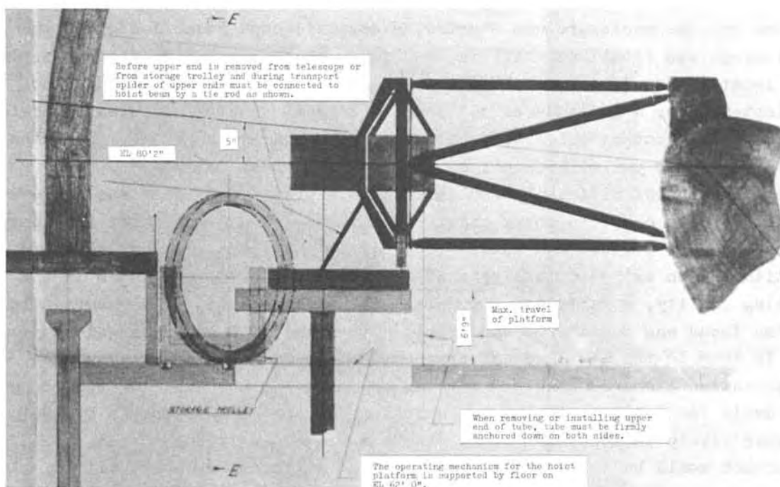
Fig. 10 Upper-end assembly.
