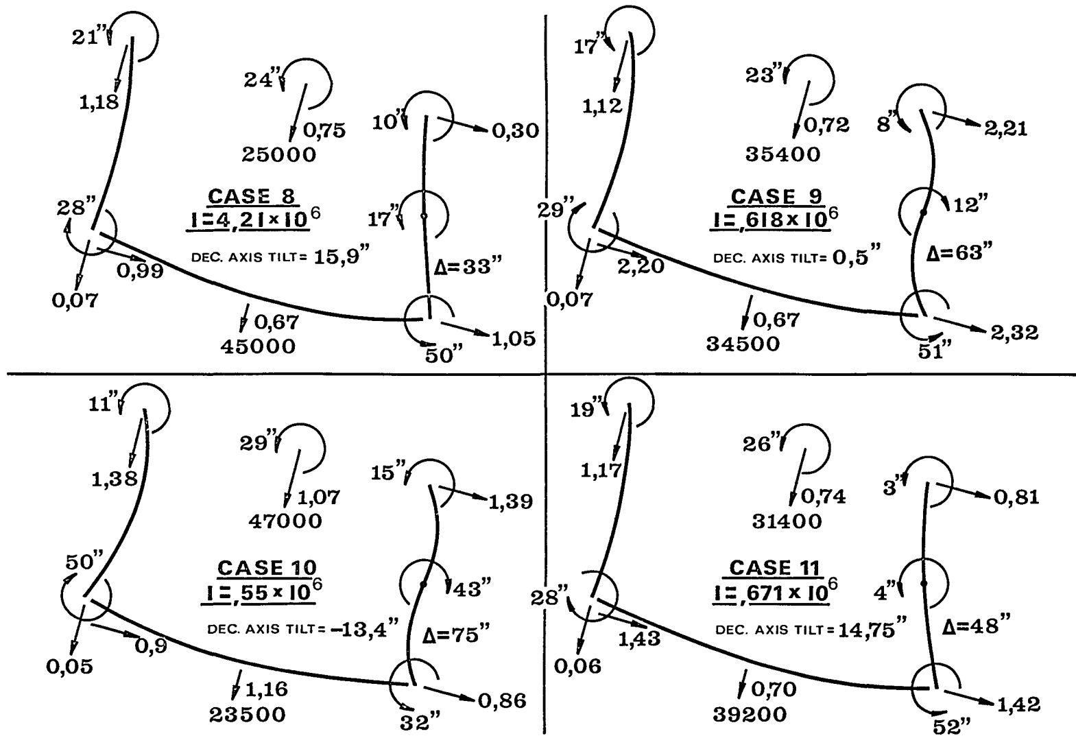
Fig. 8 Frame distortions.
