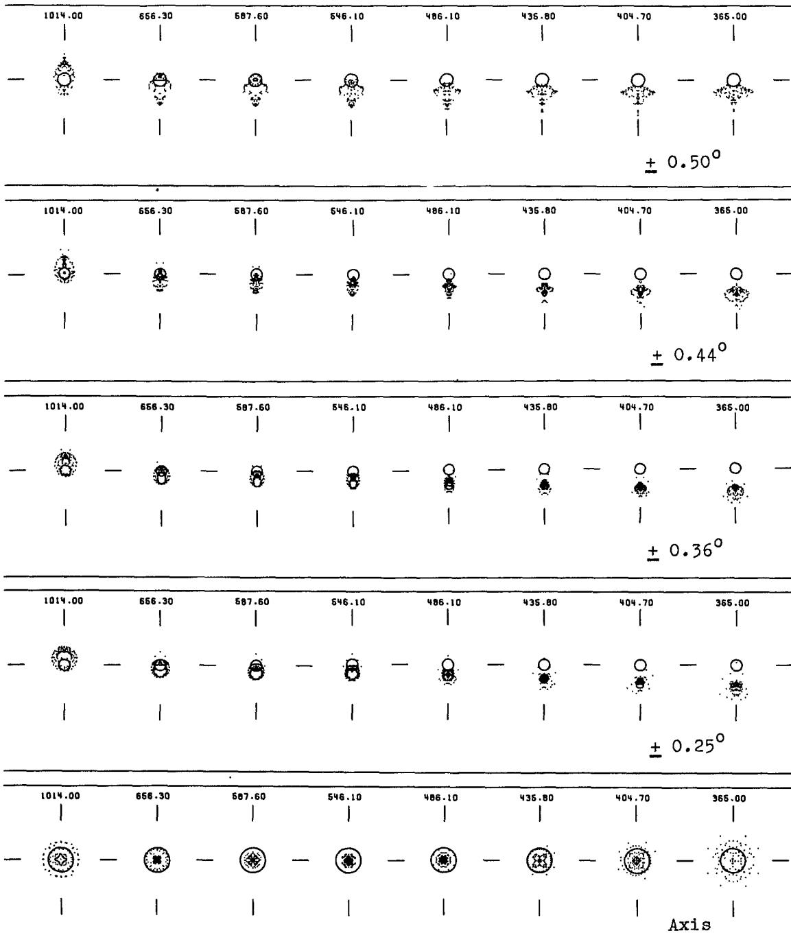
Fig. 26 Focal reducer for 3.5 m telescope. Doublet corrector ( corrected intermediate image), field lens and Bouwers-Maksutov camera. Spot diagrams. (Circle = 0.50 arcsec = 14/u.) Reduction f/8 to f/1.7. Image radius = 1066 mm.
