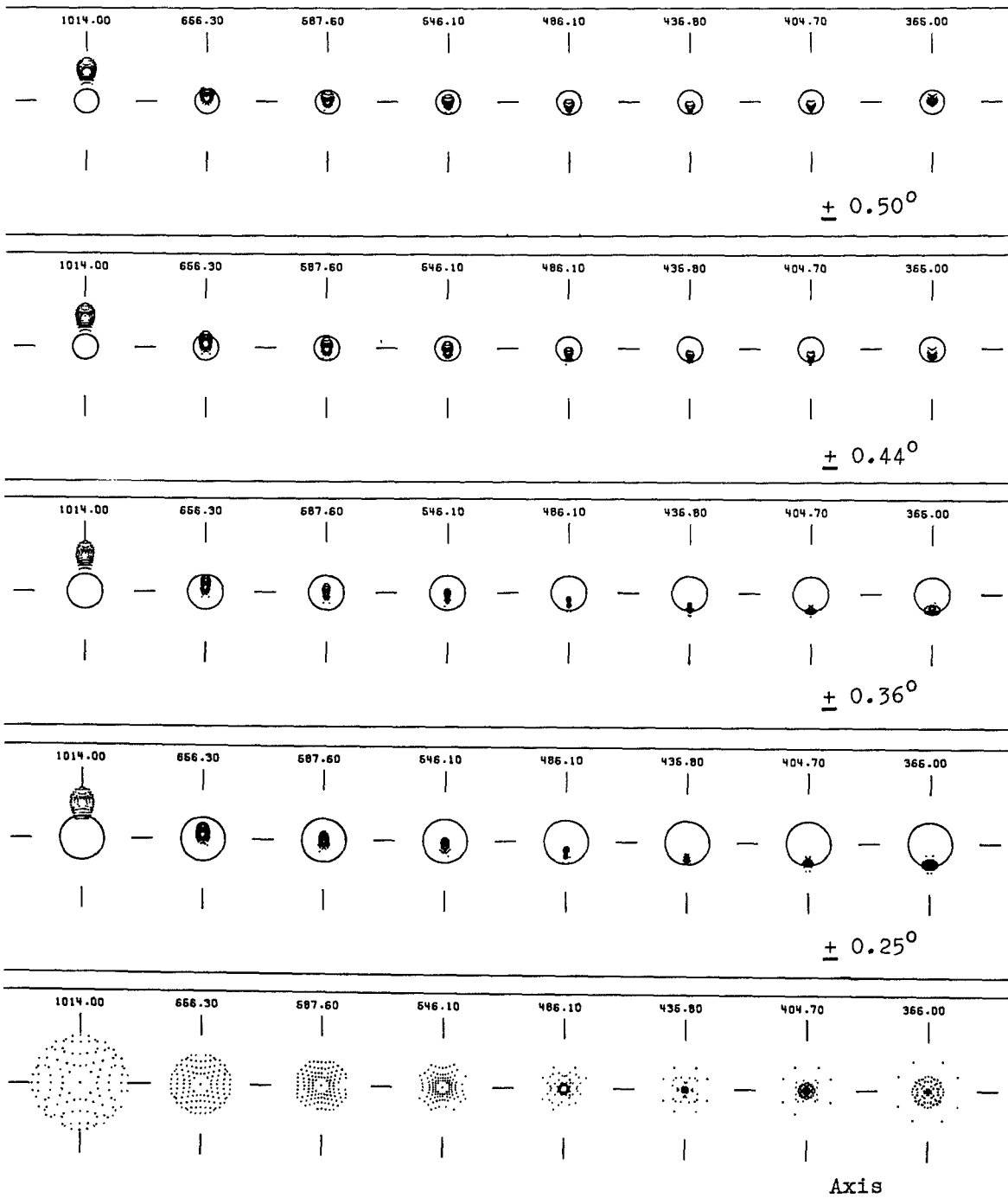
Fig. 30 Focal reducer for 3.5 m telescope. Doublet corrector ( uncorrected intermediate image), field mirror and Baker-type camera with 2 menisci and 1 plate. Spot diagrams. (Circle = 0.50 arcsec = 14/u.) Reduction f/8 to f/1.7. Image radius = 528 mm. (Plot field for axial spot diagrams = 12/u.)
