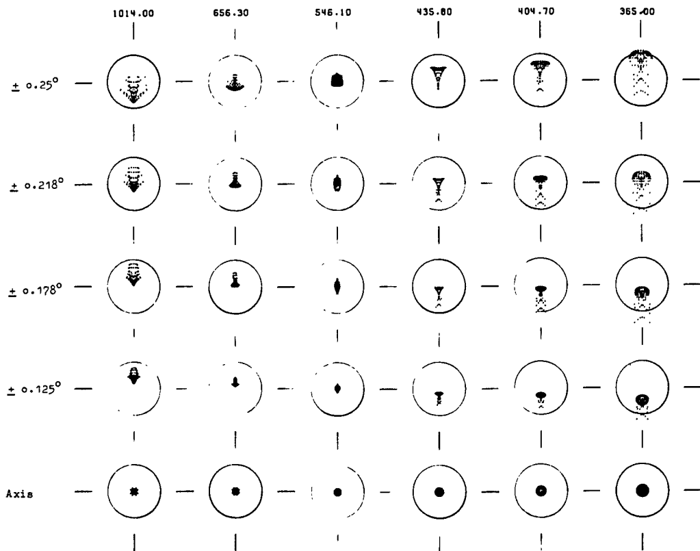
Fig. 13 3.5 m quasi Dall-Kirkham telescope (spherical secondary) with corrector of Fig. 12. Field \pm 0.25^\circ . Spot diagrams. (Circle = 0.50 arcsec = 68/μ)
