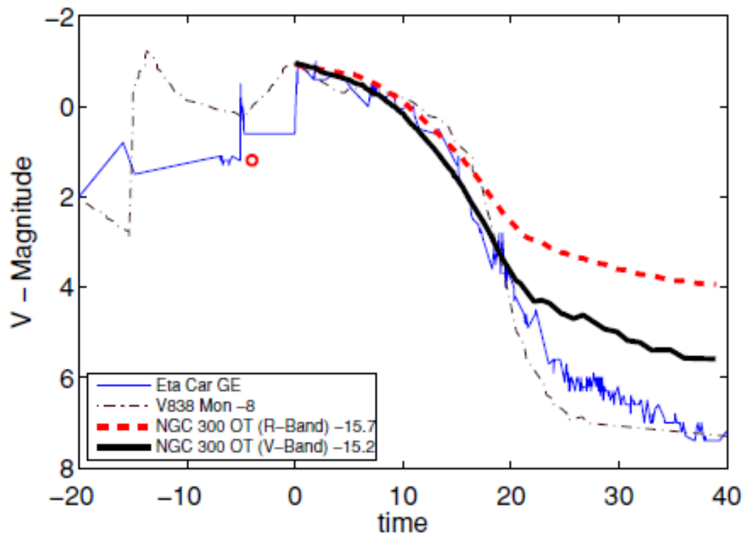
Figure 1. Comparison of the V-band light curves of the \eta Car GE, V838 Mon and NGC 300 OT. The timescale was normalized so that 1 time unit equals 1 yr for \eta Car GE, 2.2 days for V838 Mon, and 5.6 days for NGC 300 OT. For NGC 300 OT the R-band is also plotted, for which there has been one observation before the maximum (Bond et al. 2009), marked with a red circle. Top: the three separated light curves; the apparent V-mag axis was not rescaled. Bottom: the same curves translated vertically to bring peak luminosities to overlap (see legend for the shift values). It can be easily seen that the slope of the decline phase and its rate of change are similar for the three eruptions.
