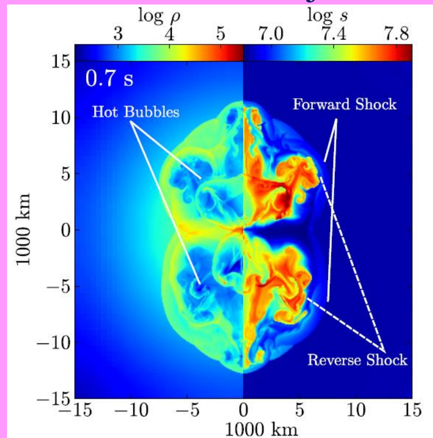
0.7 seconds of jets
