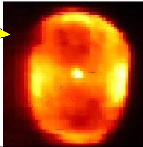
V 171 (H \alpha ) Sahai
