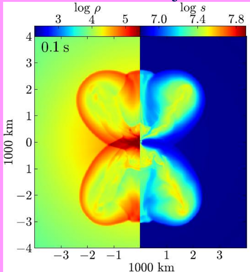
0.1 seconds of jets
