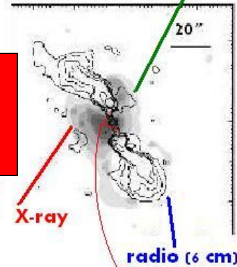
Hydra A (CF cluster) Mcnamara et al.
