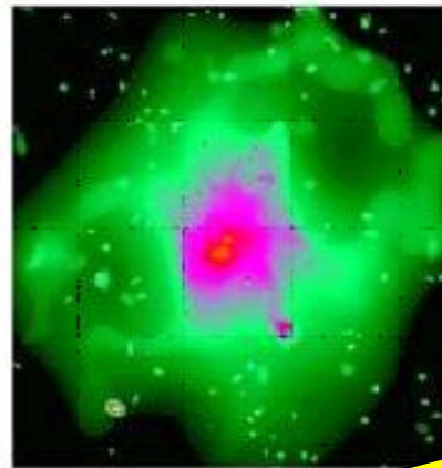
HCG 62 (X-ray) compact galaxy group Vrtilek et al.
