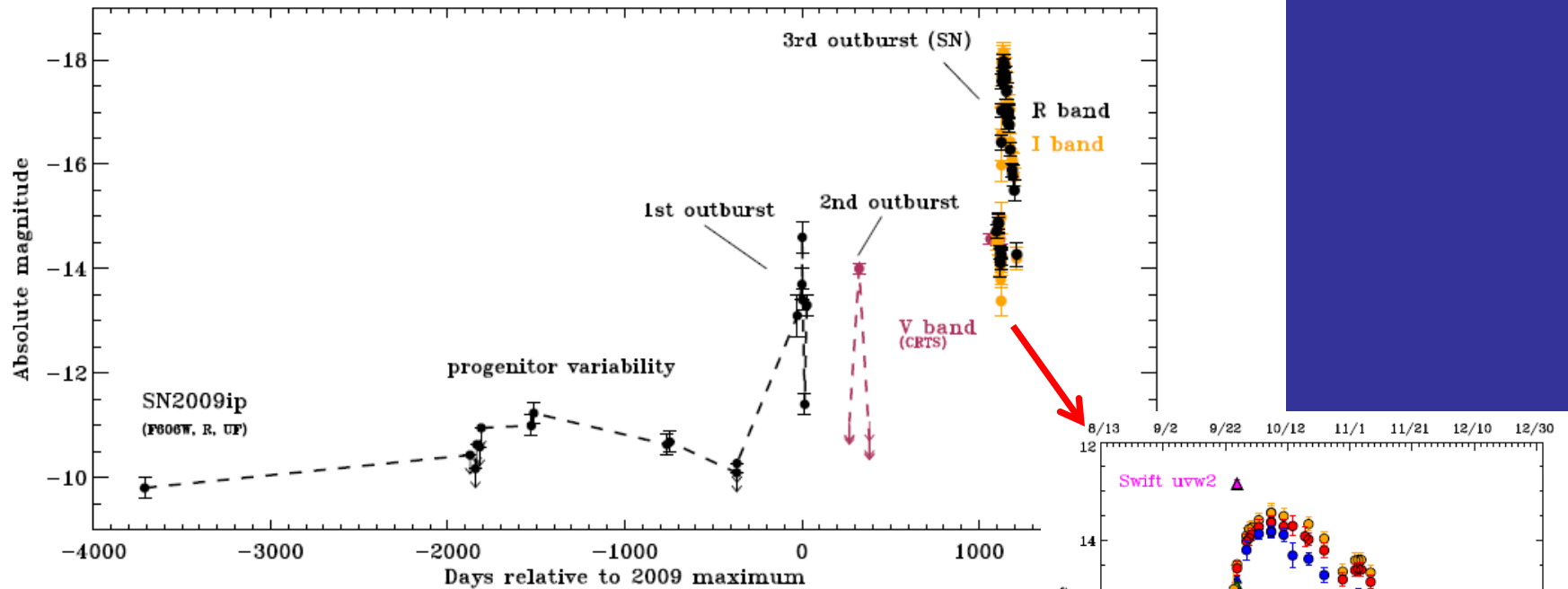
Figure 3. Absolute magnitude light curve of SN 2009ip, including archival HST data, and the ground-based photometry (see Smith et al. 2010b).
