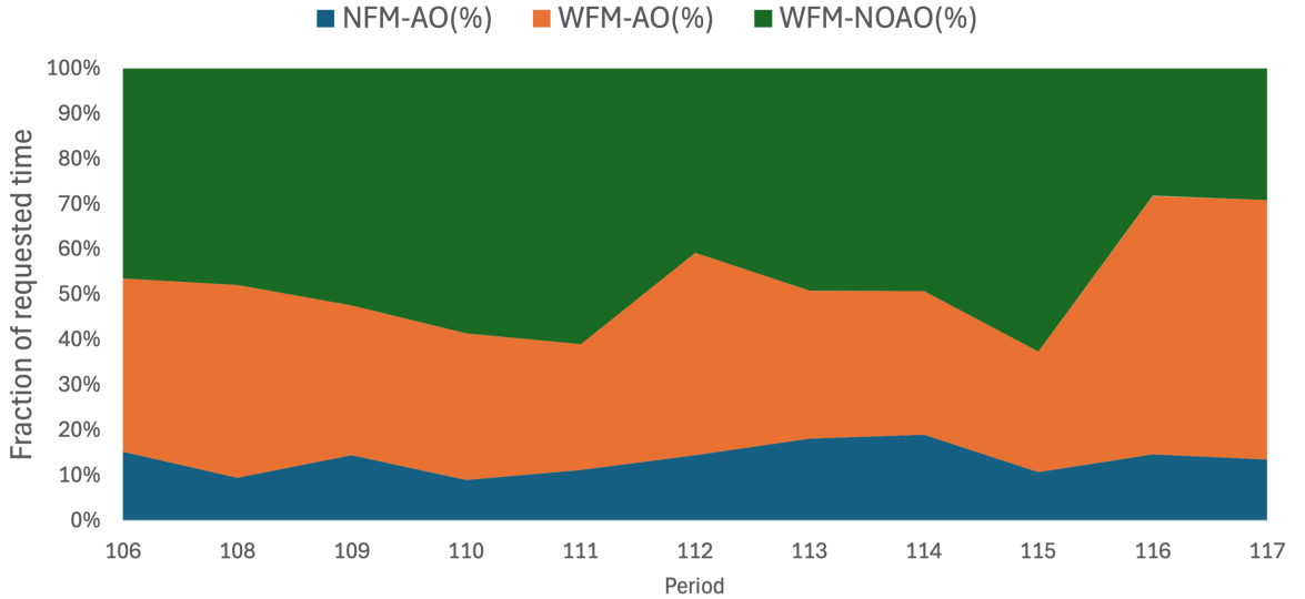
Figure 2: The fraction of requested time for MUSE observations in different modes: Narrow Field Mode (NFM-AO), Wide Field Mode with AO (WFM-AO), and Wide Field Mode with no AO (WFM-NOAO). In P116 the demand for MUSE AO modes has reached a peak above 70% of the MUSE requested time.
