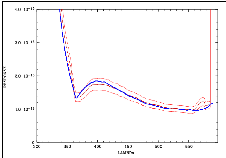
Figure 3. Propagation of master response curve back into 2009-2012. For the UVB arm, we show the average of all selected response curves from the pre-2013 period (plotted as thin red line), and its \pm 10\% envelope. The scaled master response curve from 2013 is overplotted in blue.
