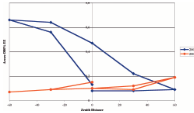
Figure 2: Coma Variation with Zenith Distance.
