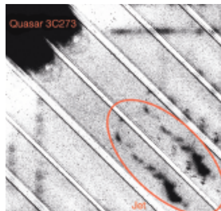
Figure 10 (below): Polarization data of the quasar 3C273 jet. NACO has been rotated to align the jet with the Wollaston stripe mask. The retarder plate can be used to turn the polarization direction in order to derive the polarization map (image prepared by Sebastian Jester).
