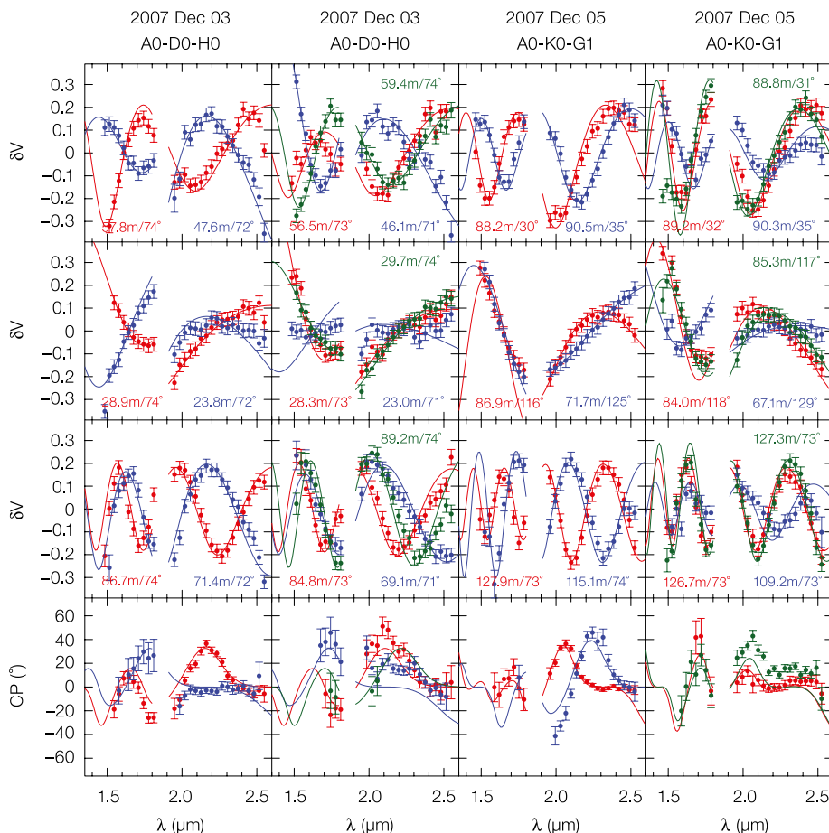
Figure 2. VLT/AMBER data obtained on \theta^1 OC during two half-nights in December 2007 (points), overlaid with our best-fit binary model. The upper three rows show wavelength-differential visibilities, while the bottom row shows the recorded closure phases.
