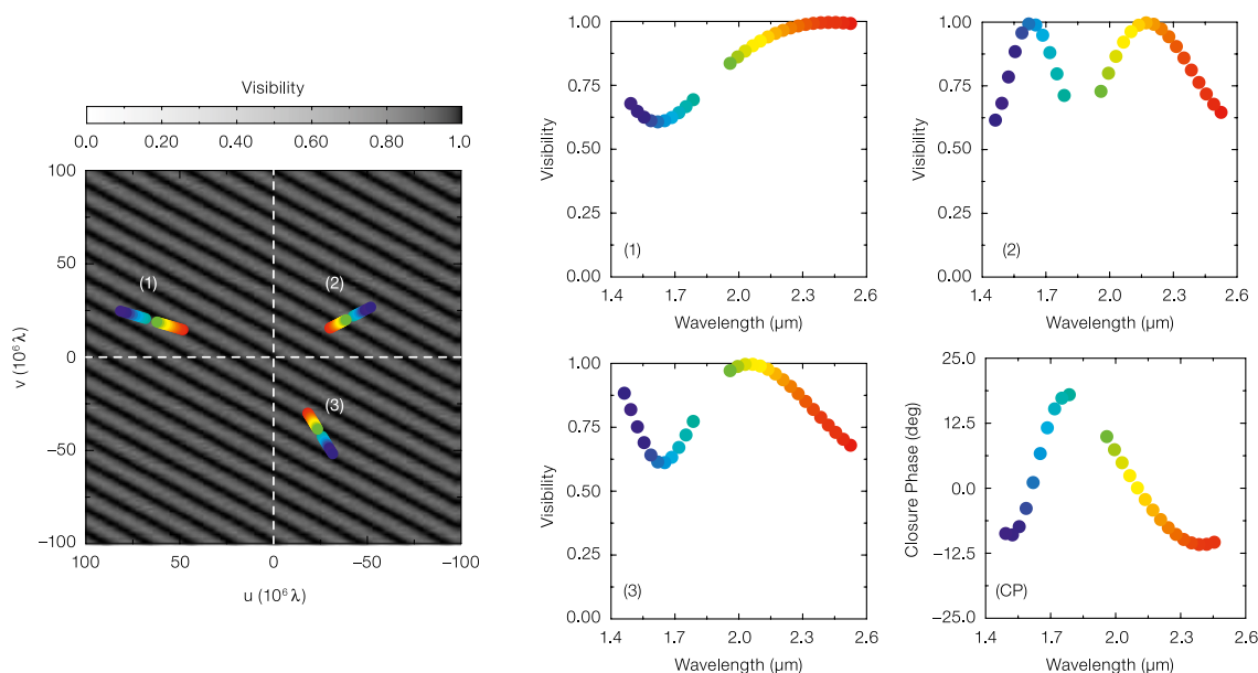
Figure 1. VLTI/AMBER three-telescope spectro-interferometry allows one to cover simultaneously the H- and K-band spectral window, resulting in radial tracks in the uv-plane (left). These radial tracks allow one to sample the sinusoidal visibility and closure phase modulation expected for a binary star, such as \theta^1 Ori C with a single AMBER observation (middle and right columns).
