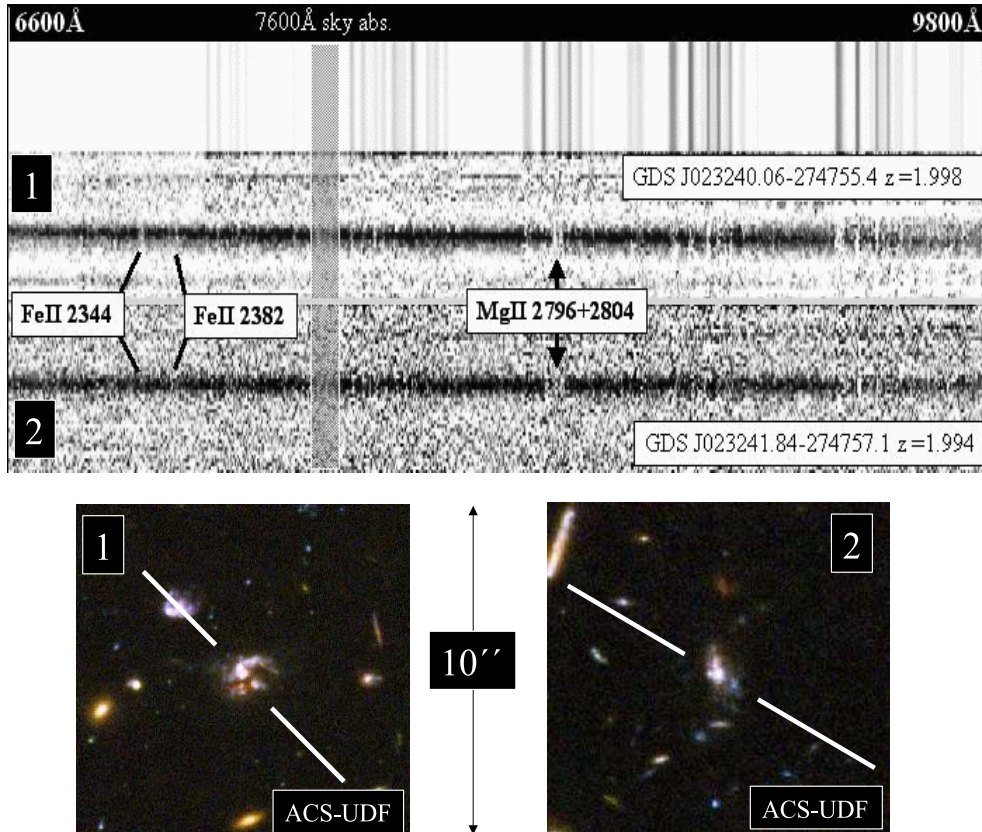
Fig. 6. Two galaxies at z=2 identified with absorption lines Mg II 2798,2802Å and [Fe II] 2344,2383Å (see text). In the top part the two dimensional spectra of the sources and the sky lines are shown. The bottom part shows the ACS-UDF color images. The solid lines indicate the orientation of the slit.
