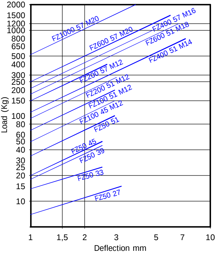
LOAD DEFLECTION CURVE FZ + Sylomer® Mounts
