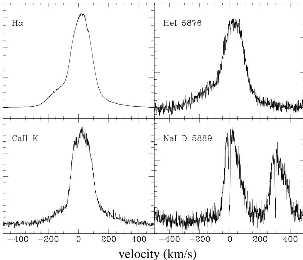
Fig. 1. Profiles of the H\alpha , HeI 5876, CaII K, and NaI D lines. The profiles of the remaining Balmer lines is virtually identical to that of H\alpha . The vertical axis has been adjusted to properly display each spectral line and is not representative of the relative fluxes.
