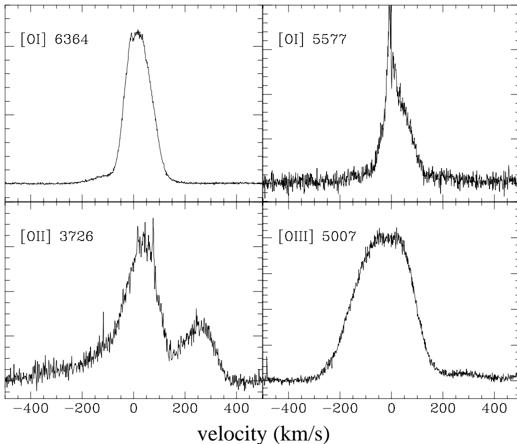
Fig. 2. Profiles of the main oxygen lines, representing in the top panels two different initial levels of the [OI] atom with very different critical densities, 1.5 \times 10^6 \text{ cm}^{-3} for \lambda = 6364 \text{ \AA} and 9.6 \times 10^7 for \lambda = 5577 \text{ \AA} . The strongest forbidden lines of singly and doubly ionized oxygen are plotted in the bottom panels. The peak to the right of the [OII] 3726 line corresponds to the [OII] 3729 line. Note the very broad profile of the [OIII] 5007 line. The sharp peak near rest velocity in the [OI] 5577 line is an artifact caused by subtraction of the strong telluric line at that position. The vertical axis has been adjusted to properly display each spectral line and is not representative of the relative fluxes.
