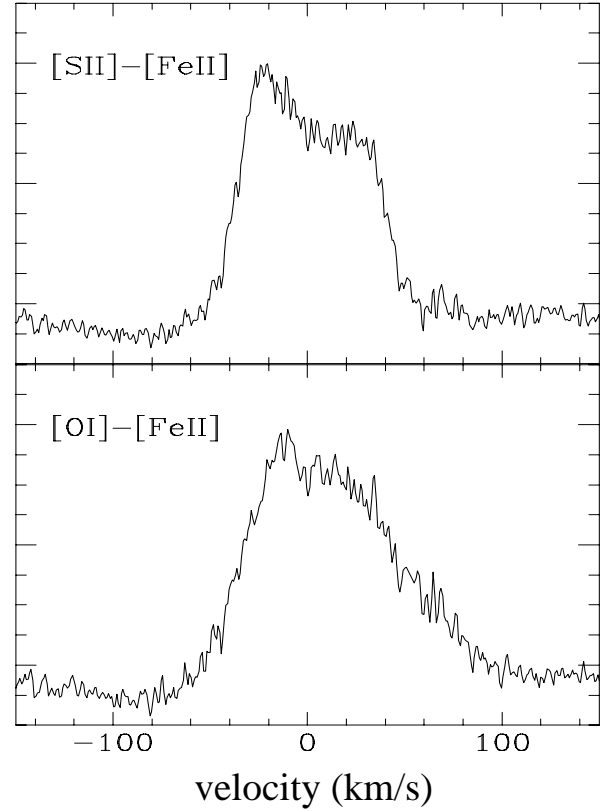
Fig. 4. Residual profiles of the [SII] 6731 (top) and [OI] 6364 (bottom), after subtraction of the profile of the [FeII] 5159 shifted to the same velocity interval and scaled by a factor such as to remove the contribution of the redshifted outflow (Sect. 4.1). The slight depression to the right of the features is caused by subtraction of the extended blue wing of the [FeII] line, which is proportionally more intense than the blue wings of the [SII] and [OI] lines. The contribution of the redshifted outflow is well removed from the spectra of the [SII] lines, but it cannot be removed from the [OI] lines at velocities below 100 km s ^{-1} .
