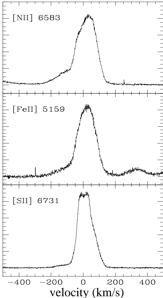
Fig. 3. Profiles of the strongest forbidden lines of [NII], [FeII], and [SII]. See also Fig. 2 for comparison with the forbidden lines of oxygen. The vertical axis has been adjusted to properly display each spectral line and is not representative of the relative fluxes.
