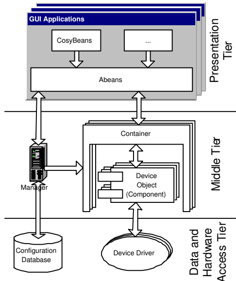
Figure 1: ACS architecture.
