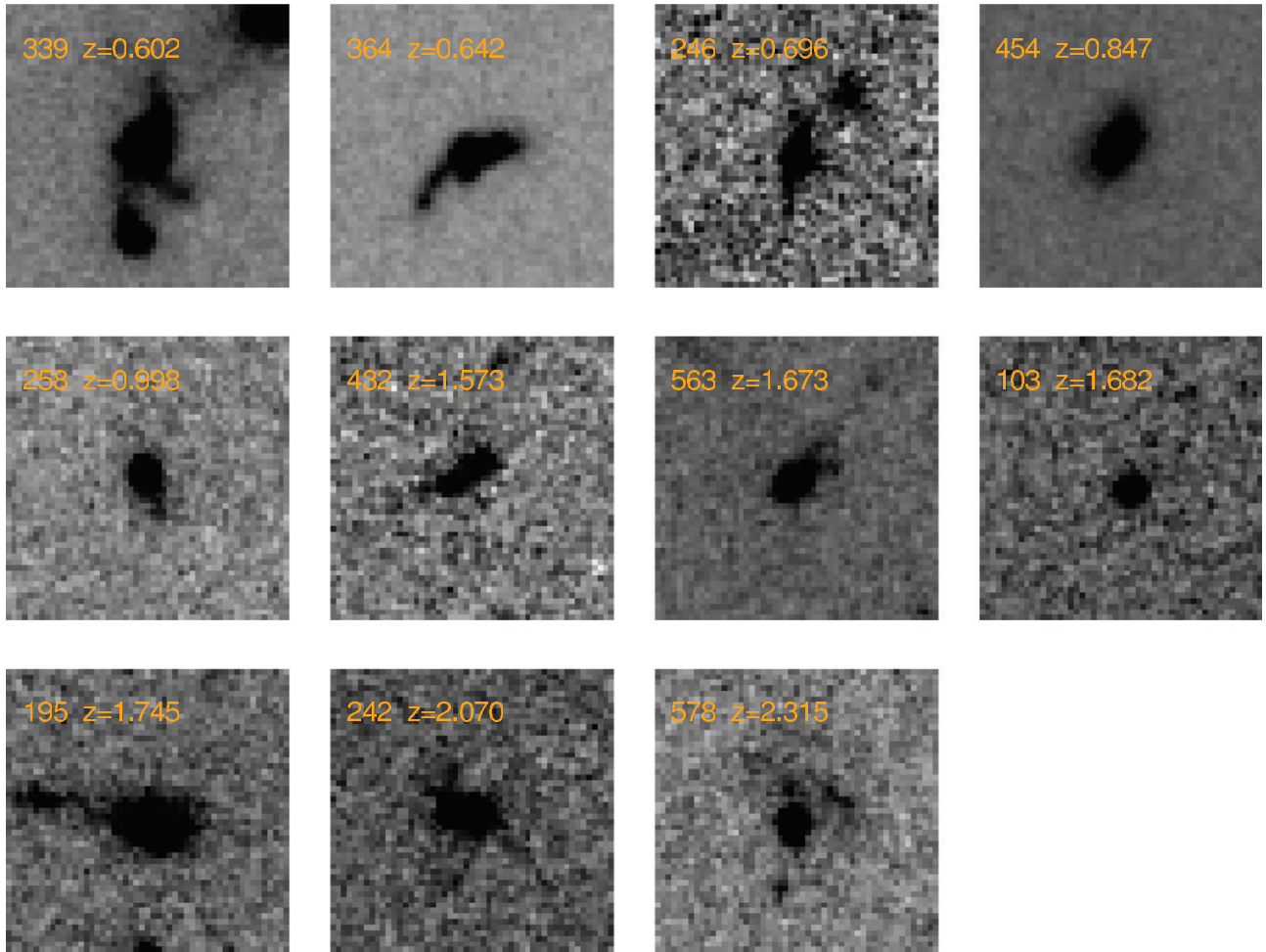
Figure 3. GOODS-S i -band postage stamps of the 11 ERS galaxies in our sample. The irregular morphologies, interacting companions, and tidal features demonstrate the ongoing star formation of these galaxies.
