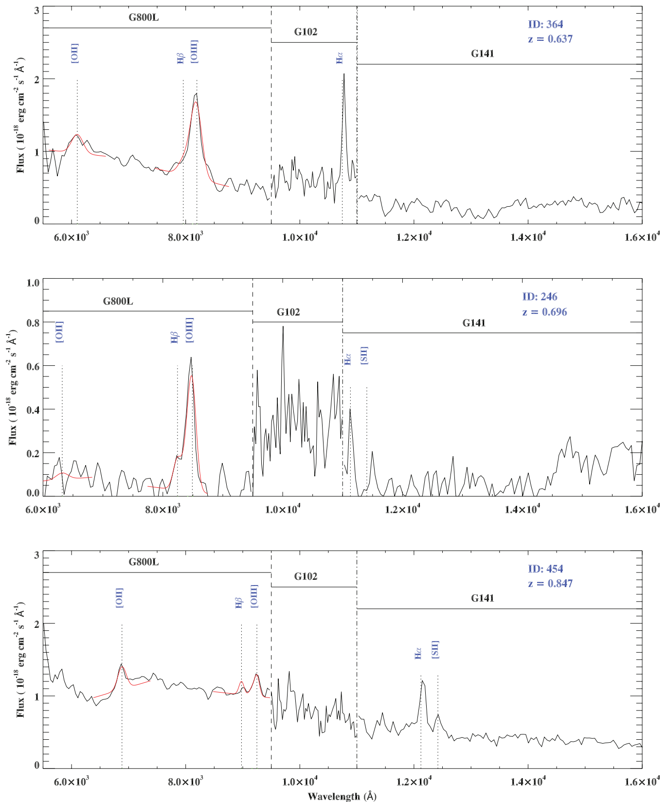
Figure 2. Example of composite grism spectra from the HST /ACS PEARS G800L grism spectroscopy and the HST /WFC3-IR ERS G102 and G141 grism spectroscopy. The emission lines [O II] \lambda 3727 , H\beta , and [O III] \lambda 5007 , H\alpha , and [S II] are detected. The H\beta and [O III] doublet are detected in both G800L and G102 grisms, and the G102 grism resolves the [O III] \lambda\lambda 4959, 5007 . The fitting of the [O III] doublet is constrained to make the ratio of the [O III] \lambda 4959 to [O III] \lambda 5007 fluxes 1:3 and to use the same line width for both. The detection of both [O II] and [O III] in the composite spectra enables the metallicity measurement using the R23 method. (A color version of this figure is available in the online journal.)
