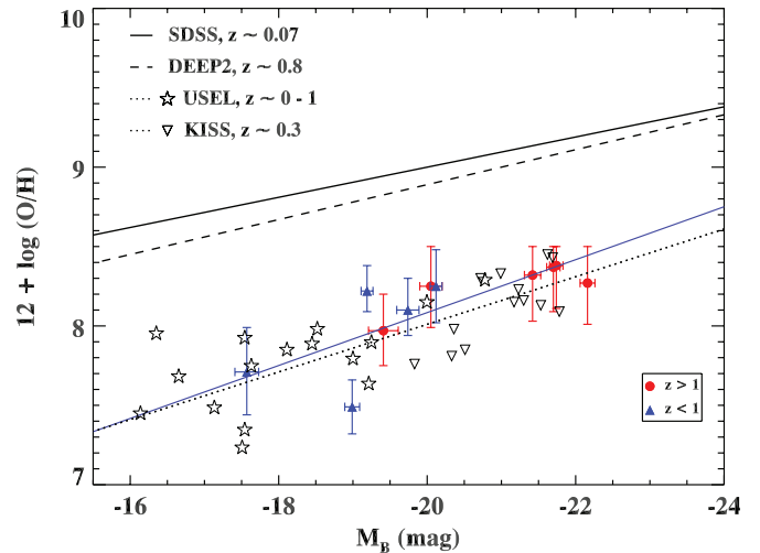
Figure 6. L – Z relation between the rest-frame B -band absolute magnitude vs. the oxygen abundance for the 10 ELGs at 0.6 < z < 2.4 . The metallicity is derived from the R23 indicator and the x -axis is the rest-frame B -band absolute magnitude. The red solid dots represent the galaxies with z > 1 , and the blue triangles represent the galaxies with z < 1 . The solid line represents the relation obtained by Tremonti et al. (2004) for SDSS star-forming galaxies at z \sim 0.1 . The dashed line illustrates the relation obtained by Zahid et al. (2011) for DEEP2 galaxies at z \sim 0.8 . The dotted line and the empty stars show the relation obtained by Hu et al. (2009) for USEL galaxies at z = 0 - 1 . The empty upside down triangles are that of Salzer et al. (2009) for [O III]-selected z \sim 0.3 galaxies. The blue solid line shows the best linear fit of our sample, which gives a relationship of 12 + \log(\text{O}/\text{H}) = (4.75 \pm 0.86) - (0.17 \pm 0.04)M_B . The PEARS sample shows an offset by about -0.6 dex in metallicity relative to the local relation at z \sim 0.1 .
