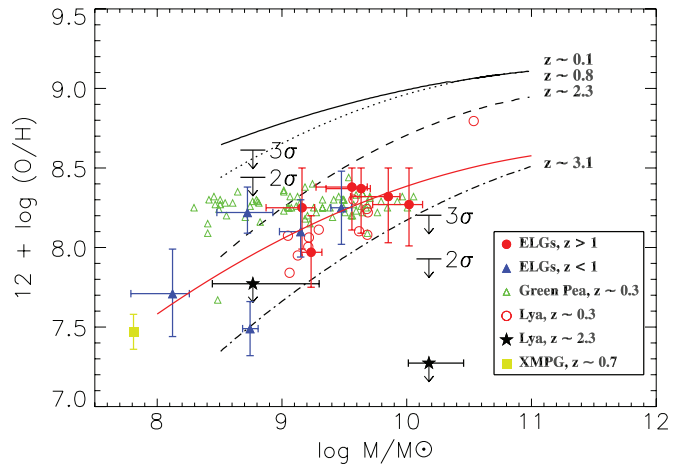
Figure 7. Relation between the stellar masses and the gas-phase oxygen abundances for our sample of 11 ELGs from PEARS and ERS grism data at 0.6 < z < 2.4 . The metallicities are estimated from the R23 method. The stellar masses are estimated from the SED fitting with BC03 model and have been scaled to a Chabrier (2003) IMF to be consistent with other studies. The definition of the points of our sample are the same as Figure 5. Also plotted for comparison are the green peas (empty green triangles) at z \simeq 0.3 (Amorin et al. 2010), \text{Ly}\alpha galaxies at z \simeq 0.3 and z \simeq 2.3 (Finkelstein et al. 2011a, 2011b), and the WISP XMPG galaxy at z \simeq 0.7 (Atek et al. 2011). The solid red line is the best fit of the M-Z relation to the 11 ELGs in our sample. The solid line represents the M-Z relation at z \simeq 0.1 from Tremonti et al. (2004) for the local SDSS galaxies. The dashed line shows the M-Z relation at z \simeq 0.8 for the 1350 DEEP2 galaxies from Zahid et al. (2011). The dotted line and the dash-dotted line are that at z \simeq 2.3 from Erb et al. (2006) and at z \simeq 3.1 from Mannucci et al. (2009), respectively. The M-Z relations at different redshifts are calibrated to the same metallicity indicator of Kobulnicky & Kewley (2004) from Zahid et al. (2011). The large offset of \sim 0.5 dex of this sample relative to the other relations at similar redshift demonstrates that these galaxies may be at the early stages of galaxy evolution. Infall of gas due to mergers is another popular explanation, e.g., Peeples et al. (2009) and Rodrigues et al. (2012). (A color version of this figure is available in the online journal.)
