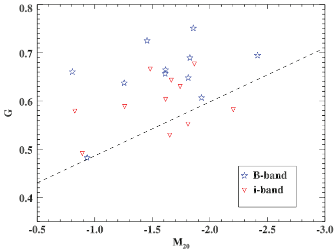
Figure 4. Gini coefficient G vs. M_{20} to demonstrate the morphology analysis of the 11 galaxies in our sample. The dashed line is the empirical line dividing interacting galaxies (upper region) with normal galaxies (lower region) from Lotz et al. (2004). The blue stars represent galaxies based on B -band image analysis. The red triangles are that based on i -band image analysis. Most galaxies lie above the line demonstrating disturbed morphologies.
