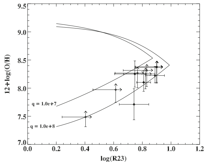
Figure 5. \log(R23) vs. oxygen abundance for the 11 ELGs in our sample. The overplotted lines represent the theoretical lines at q = 1.0 \times 10^7, 1.0 \times 10^8 (Kobulnicky & Kewley 2004). All of the galaxies are put on the lower branch according to the branch criteria. The 3\sigma upper limit of the \text{H}\beta line fluxes give the lower limit of \log(R23) and hence the lower limit of 12 + \log(\text{O}/\text{H}) at the lower branch, which are shown as arrows.
