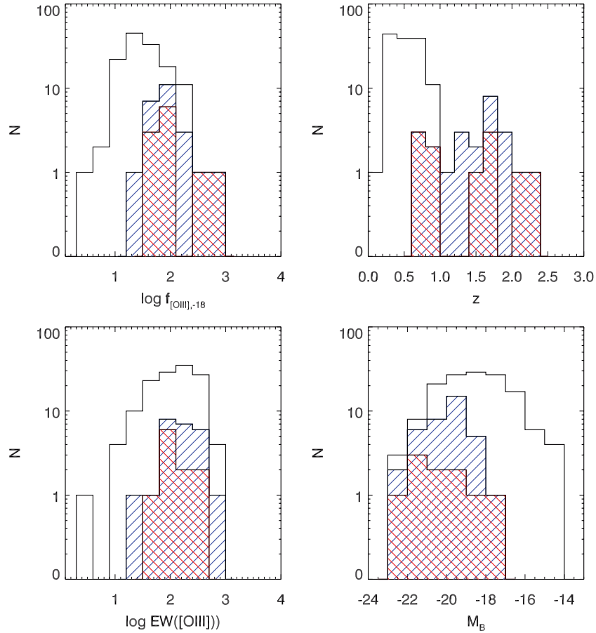
Figure 1. Histogram distributions of the [O III] line fluxes ( f_{[\text{O III}]-18} = f_{[\text{O III}]} / 10^{-18} \text{ erg cm}^{-2} \text{ s}^{-1} ), the equivalent widths (EWs), redshifts, and the absolute B -band magnitudes of the 11 ELGs from the combined catalog (red -45 deg tilted line filled) with respect to the Straughn et al. (2009) PEARS ELG sample (empty black solid line) and the Straughn et al. (2011) WFC3 ERS ELG sample (blue 45 deg tilted line filled).
