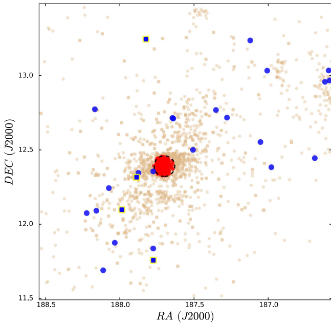
Figure 4. Spatial distribution of the GC sub-samples defined in Figure 3.
