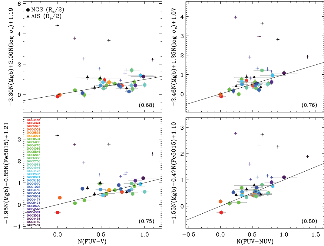
Figure 6. Edge-on views of the best-fitting planes for selected three-parameter relations (see text). Top left-hand panel: plane relating FUV - V , Mgb and \sigma_e . Bottom left-hand panel: plane relating FUV - V , Mgb and Fe5015 . Top right-hand panel: plane relating FUV - NUV , Mgb and \sigma_e . Bottom right-hand panel: plane relating FUV - NUV , Mgb and Fe5015 . The solid lines are shown to guide the eye and all have slope unity and go through the origin. The correlation coefficient is reported in the bottom right-hand corner of each panel. The three-parameter correlations shown are not tighter than the two-parameter correlations shown in Figs 1 and 4.
