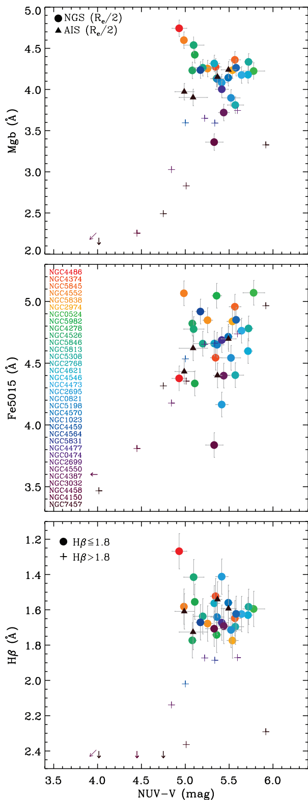
Figure 3. Same as Fig. 1 but for the optical–UV colour ( \text{NUV} - V ).
