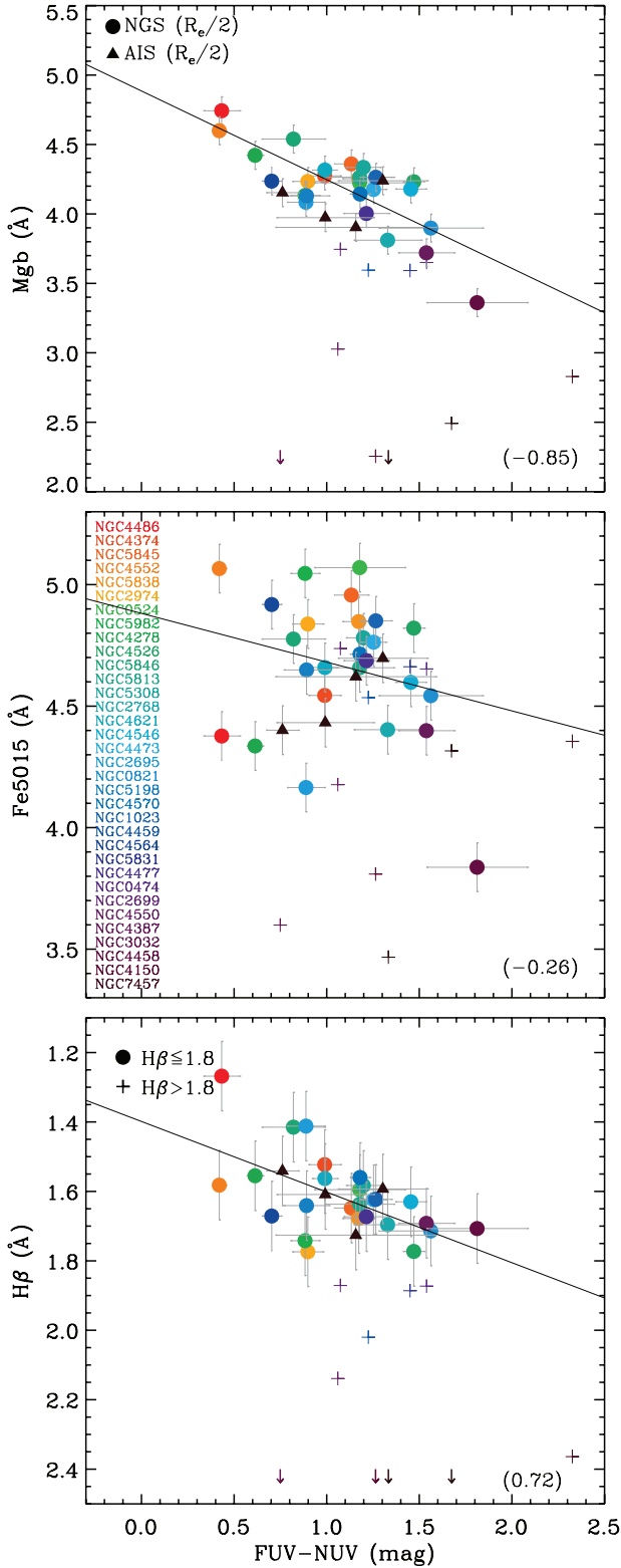
Figure 4. Same as Fig. 1 but for the pure UV colour ( FUV - NUV ).
