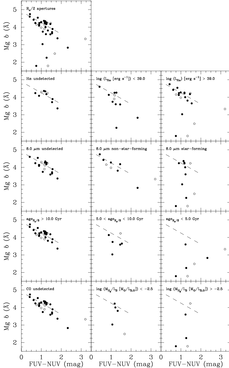
Figure 7. Dependence of the (FUV - NUV) – Mg\,b correlation on recent and ongoing star formation. The top panel shows the correlation for all galaxies using elliptical apertures of R_e/2 . Lower panels show the correlation as a function of the integrated H\alpha luminosity, the type of 8.0\,\mu\text{m} non-stellar emission if present, the luminosity-weighted mean stellar age and the molecular gas mass normalized by the B -band luminosity. From left to right, the columns respectively show galaxies with no, mild or ambiguous and strong evidence for ongoing or recent star formation. A clear correlation with no outlier is only observed for quiescent galaxies. Filled symbols indicate galaxies with at least one orbit of GALEX integration time, while open symbols indicate the shorter exposure AIS data. Error bars have been omitted for clarity and our best-fitting (FUV - NUV) – Mg\,b relation is overplotted as a dashed line for reference.
