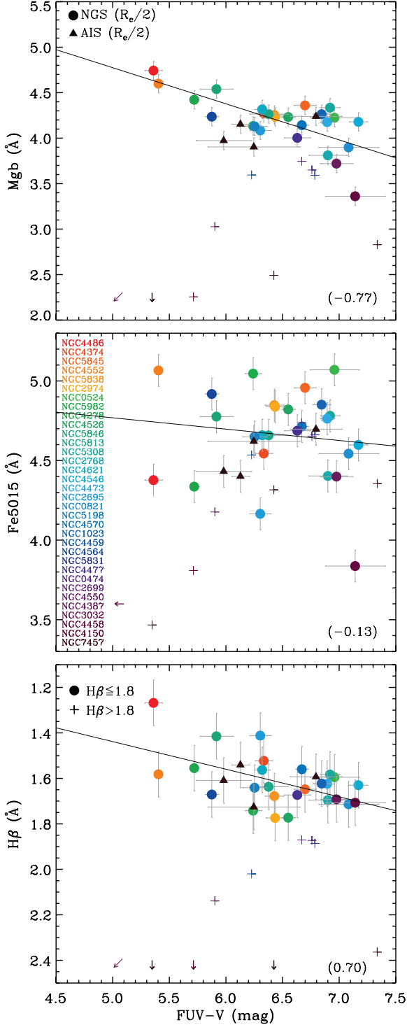
Figure 1. UV-upturn dependence on stellar absorption line strengths. The Mg\ b (top panel), Fe5015 (middle panel) and H\beta (bottom panel) line strengths are shown as a function of the FUV - V colour, all integrated within R_e/2 . The top panel is our own version of the Burstein relation. Objects inconsistent with a purely old stellar population ( H\beta > 1.8\ \text{\AA} ) are plotted as crosses, others as filled circles. The location of data points lying outside the figure boundaries is indicated by arrows. Note the inverted H\beta axis. Linear fits to the data with H\beta \leq 1.8\ \text{\AA} are shown as solid lines to guide the eye, and the correlation coefficient is reported in the bottom right-hand corner of each panel. The best-fitting parameters are listed in Table 2. The colour table traces the effective stellar velocity dispersion \sigma_e , from purple at small dispersions through green and red at high dispersions.
