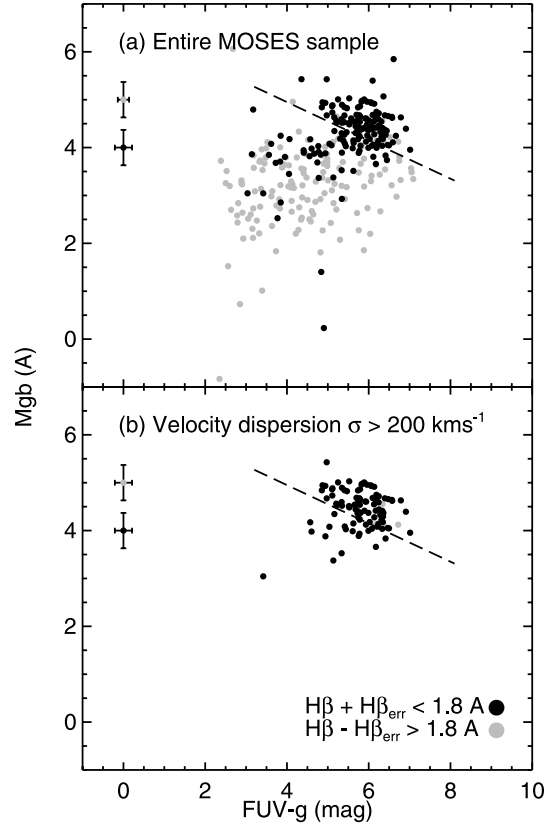
Figure 8. Mg b –( FUV - g ) relation for the MOSES sample early-type galaxies with good UV photometry. Top panel: entire sample meeting the H\beta selection criteria. Bottom panel: only galaxies with a velocity dispersion \sigma larger than 200 \text{ km s}^{-1} . Quiescent galaxies with H\beta + H\beta_{\text{err}} \leq 1.8 \text{ \AA} are shown as black circles, while galaxies consistent with harbouring a young stellar population ( H\beta - H\beta_{\text{err}} > 1.8 \text{ \AA} ) are shown in grey. Characteristic error bars are shown in the top left-hand side of each panel. Our best-fitting Burstein relation is overplotted as a dashed line for reference, taking into account the g - V colour transformation described in the text.
