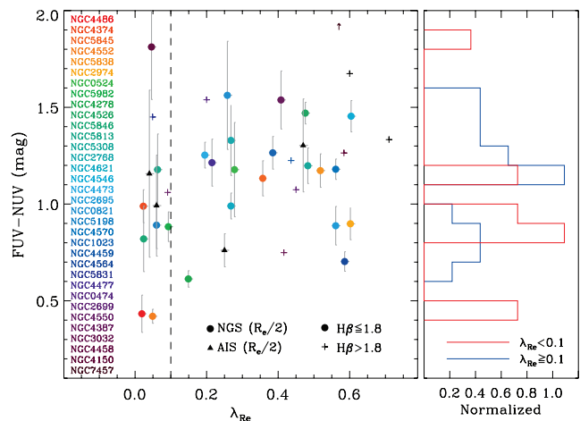
Figure 9. Same as Fig. 1 but for the FUV - NUV colour as a function of the specific angular momentum of the galaxies \lambda_{R_e} . The normalized number distribution of slow-rotator (red) and fast-rotator (blue) galaxies as a function of the FUV - NUV colour is shown on the right-hand panel for quiescent galaxies only (i.e. circles and triangles).
