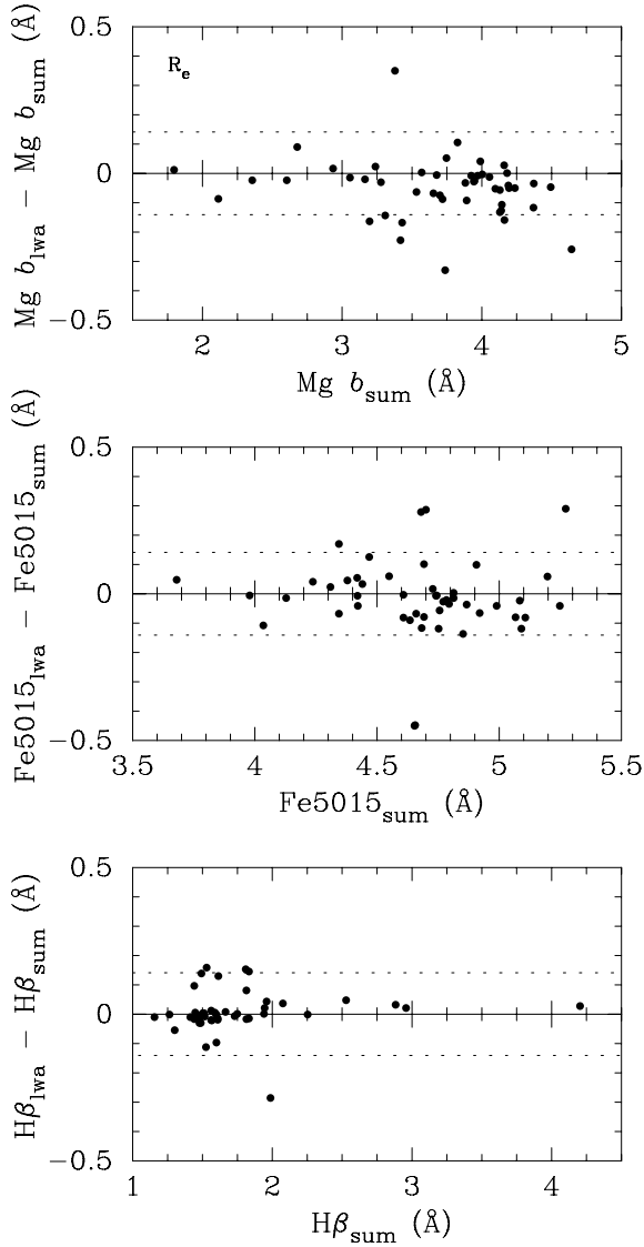
Figure A1. Comparison of integrated line-strength values obtained by properly summing the spectra (labelled ‘sum’) and simply luminosity-weighting the line-strength values themselves (labelled ‘lwa’) within circular apertures of radii R_e . Error bars are omitted for clarity, but the adopted formal random error on either quantity is 0.1 \text{ \AA} . Top panel: \text{Mg } b . Middle panel: \text{Fe5015} . Bottom panel: \text{H}\beta . The scatter is always much smaller than the range of values covered and there is no significant systematic trend. The dotted lines show the 0.14 \text{ \AA} formal random error on the difference.
