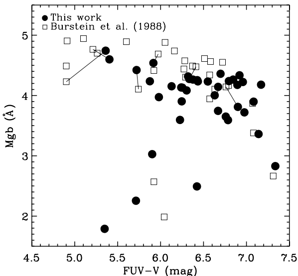
Figure 2. (FUV – V)–Mg b (i.e. Burstein) relation for both our data (filled circles) and the 1550 Å and Mg 2 data of BBBFL88 (open squares). The latter have been transformed to FUV and Mg b as discussed in the text. Galaxies in common between the two samples are connected by a solid line. Error bars have been omitted for clarity. The two data sets are consistent, with similar scatter.
