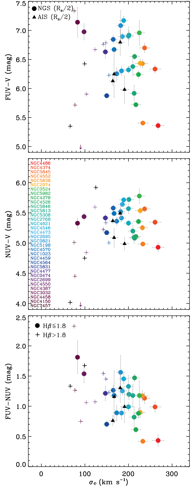
Figure 5. Same as Fig. 1 but for the FUV - V , NUV - V and FUV - NUV colours as a function of the effective stellar velocity dispersion \sigma_e .
