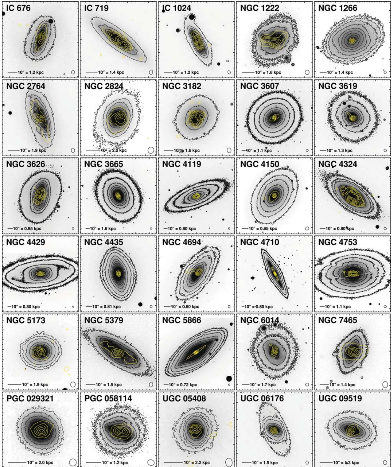
Figure 1. r -band images (grey-scale and black contours) overlaid with integrated CO(1–0) contours (yellow) at 10, 30, 50, 70 and 90 per cent of the peak intensity for the 30 galaxies in the ATLAS 3D CARMA sample. The r -band images were either taken from the SDSS or a dedicated programme with the INT (Paper XXI). The CO-synthesized beam is shown in the bottom-right corner of each panel. A bar in the bottom-left corner of each panel indicates the scale of 10 arcsec, as well as the equivalent physical scale at the distance of the galaxy.
