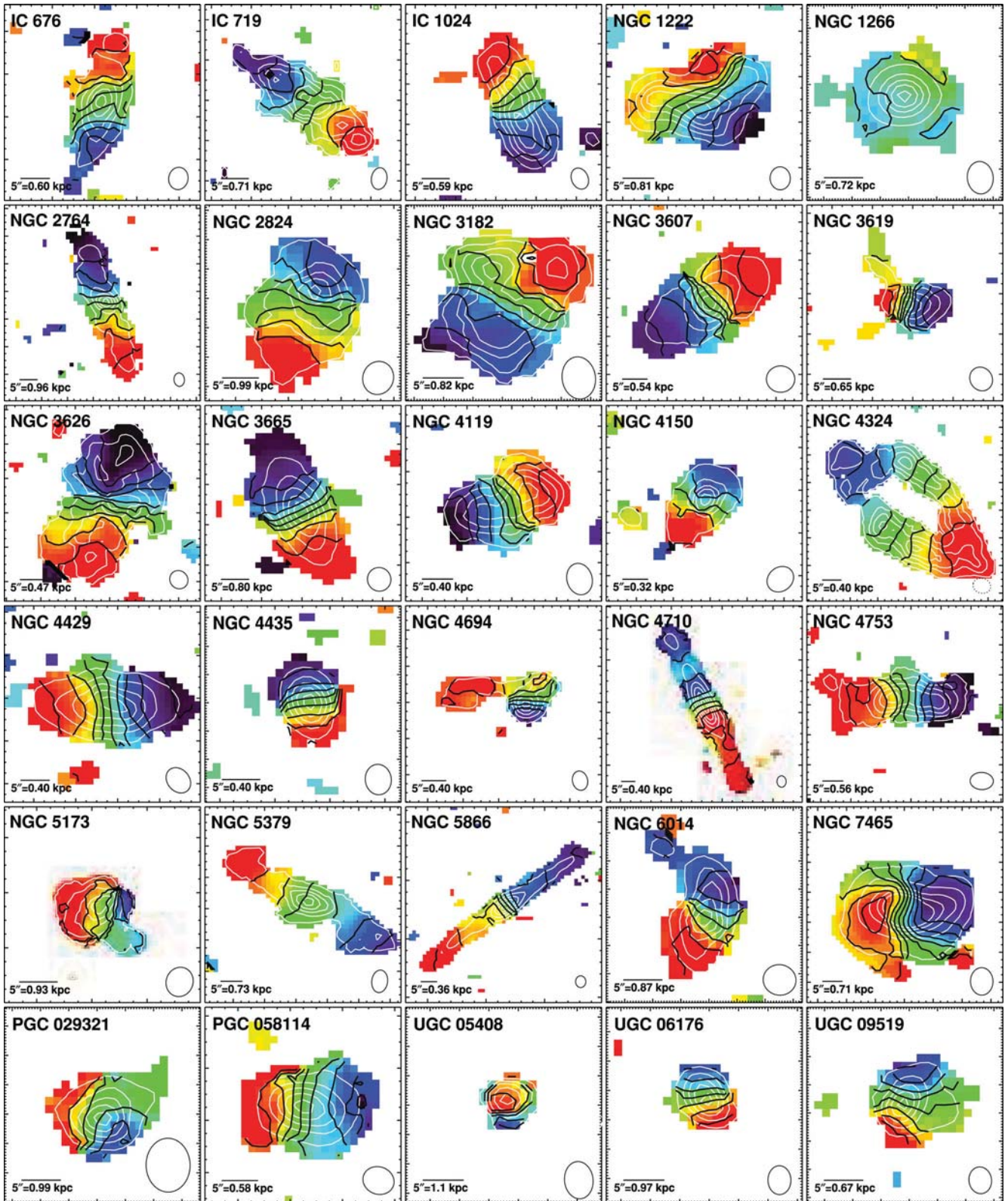
Figure 2. Mean CO(1–0) velocity maps of the 30 galaxies of the ATLAS 3D CARMA sample. Isovelocity contours (black) are overlaid at 20 \text{ km s}^{-1} intervals, as are contours from the moment0 map (white). The CO-synthesized beam is shown at the bottom-right corner of each panel. A bar in the bottom-left corner of each panel indicates the scale of 5 arcsec, as well as the equivalent physical scale at the distance of the galaxy.
