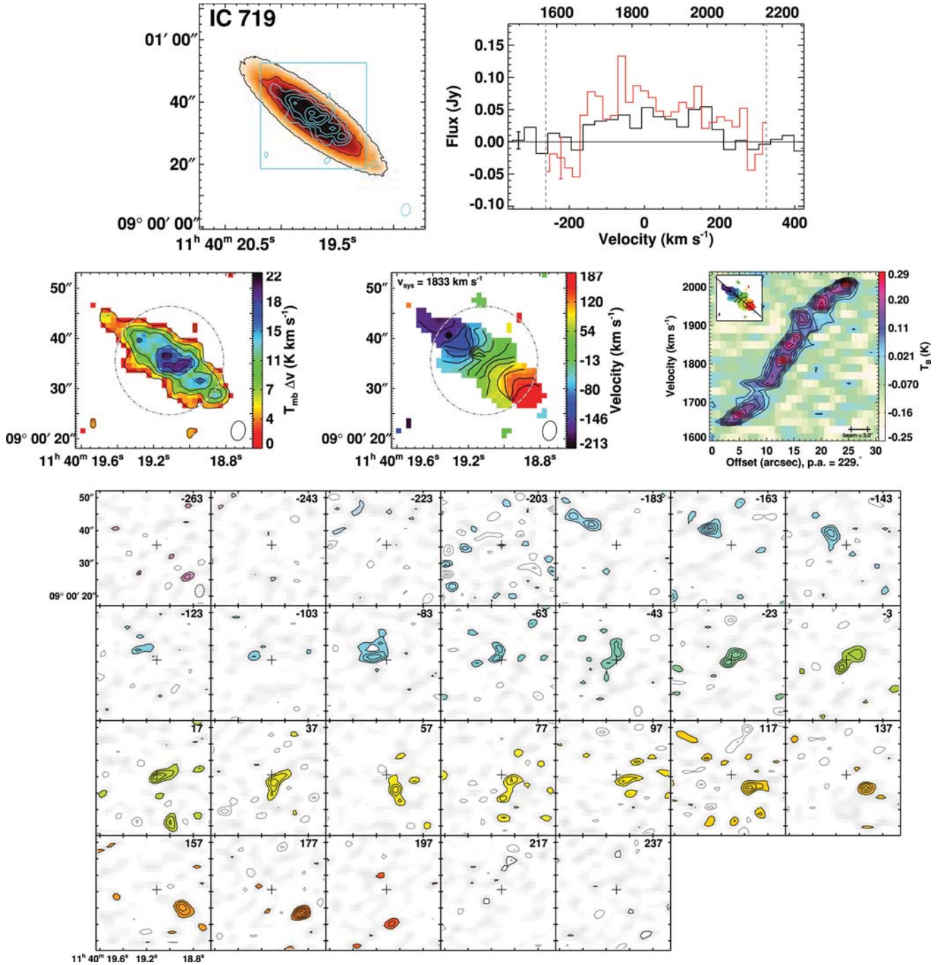
Figure A2. IC 719 is a field 2\sigma non-regular rotator ( M_K = -22.70 ) with normal stellar morphology. It contains a dusty disc. The 2\sigma peak is the signature of two counter-rotating stellar discs with opposite angular momenta. The molecular gas is corotating with a kinematically decoupled core, and counter-rotating with respect to the dominant stellar component. The moment0 peak is 2.6 \text{ Jy beam}^{-1} \text{ km s}^{-1} . The moment1 contours are placed at 25 \text{ km s}^{-1} intervals.
