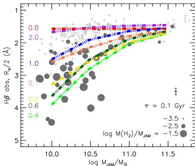
Figure 10. Similar to Fig. 4, with overlays showing the evolution of old galaxies with 3 \times 10^8 M_{\odot} of recent star formation activity. The red line marked ‘0.0’ shows the model red sequence before star formation is initiated, and subsequent lines show how H\beta changes through the late burst. Each isochrone is labelled with the time (in Gyr) since the initiation of the burst.
