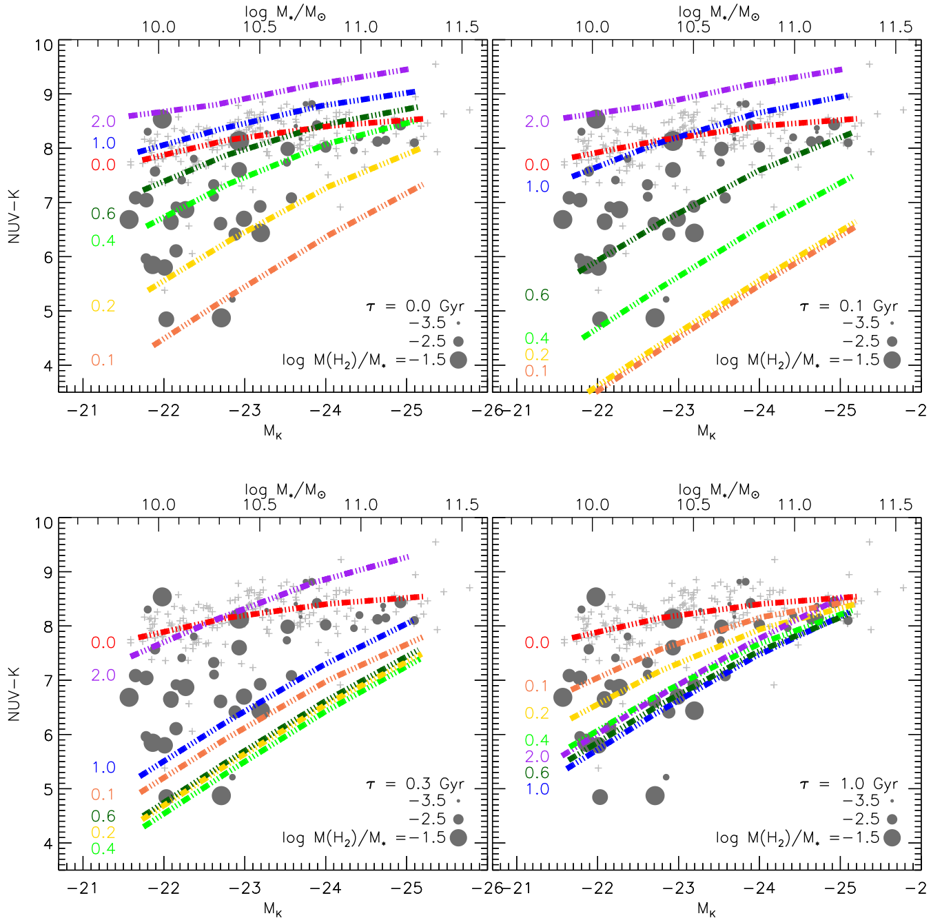
Figure A2. Similar to Fig. 8, with NUV - K model isochrones.
