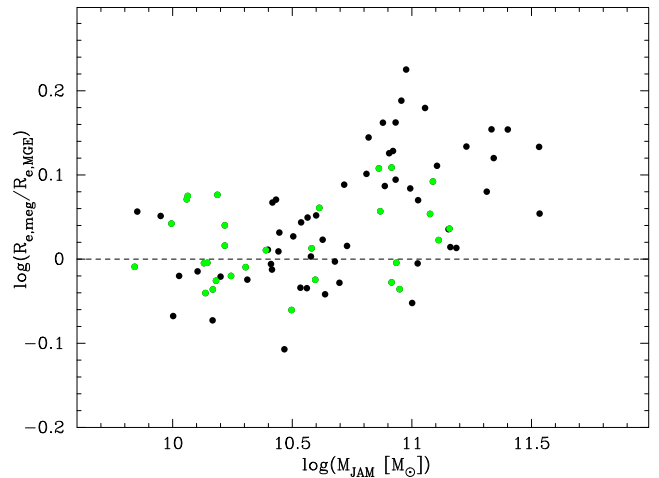
Figure 26. Ratio between the effective radius estimated with the MegaCam r band (with an ellipse fitting modelling of the ETG) and that determined from the SDSS/INT images (with MGE modelling; Cappellari et al. 2013a) as a function of the dynamical mass, M_{\text{JAM}} . Relaxed galaxies showing no sign of tidal perturbations even with the deep imaging are shown in green.
