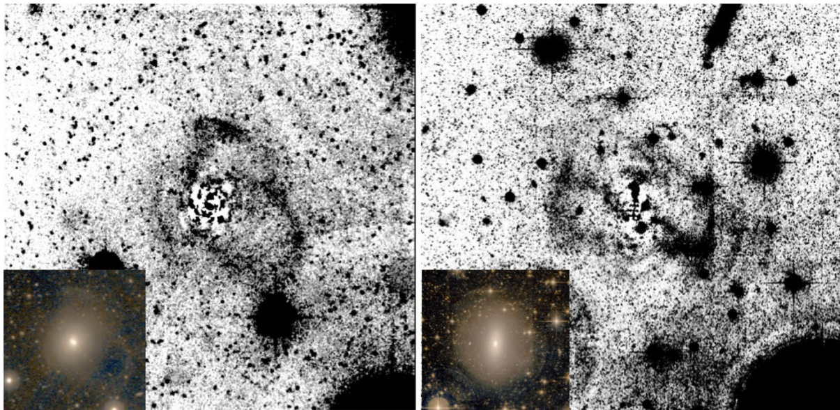
Figure 15. Examples of fine structures being revealed after subtracting a galaxy model made with ellipse fitting. Residual g -band image of UGC 05408 (left) and NGC 3245 (right). The insets show true colour g + r images of the central regions before the galaxy subtraction.
