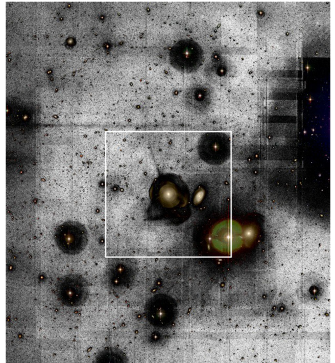
Figure 4. g -band image of the field around NGC 474. The chosen intensity scaling enhances the fainter extended LSB features, including the extended reflection haloes around the bright stars and other instrumental signatures, such as horizontal and vertical bands corresponding to lower sensitivity in the CCD gaps and at the edges of the recombined frames. On such images, non-circular or rectangular features, and oblique filaments are real structures on the sky. The target galaxy lies at the centre of the white square, the size of which corresponds to 40 times the effective radius of the ETG. To better identify the objects, a composite g + r + i image has been superimposed. The field of view of the large-scale image is 57 \times 64 arcmin 2 . North is up and east left. Similar images are provided for all our targets in the image catalogue.
