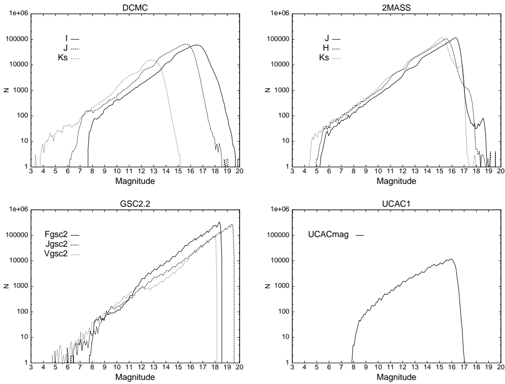
Fig. 1. Completeness diagrams for four major surveys covering the LMC. Each plot gives the number of sources per magnitude bin. The bin size is 0.1 magnitude. Note that: 2MASS observations (upper right) are deeper than DENIS observations (upper left) in the K_S band; the GSC2.2 magnitudes (bottom left) show a sharp cut-off ; the UCAC1 magnitudes (bottom right) are only indicative, since the UCAC1 is not a photometric catalogue and furthermore this is only a preliminary catalogue, which means some improvements are expected in future releases.
