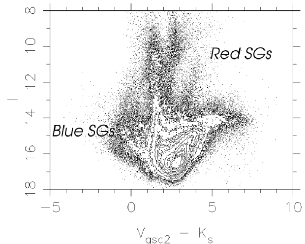
Fig. 13. Panel (a) contains sources detected by both DCMC and 2MASS: 372,354 entries. The I band is from DENIS, whereas the J and K_S bands are from 2MASS. Dwarf and giant tracks superimposed are from Bessel & Brett (1988). Panel (b) contains sources detected by both GSC2.2 and 2MASS: 147,564 entries. Dwarf and giant tracks are computed using Table 2 from Wainscoat et al. (1992). The sources involved in those diagrams have photometric errors smaller than 0.06 magnitude.
