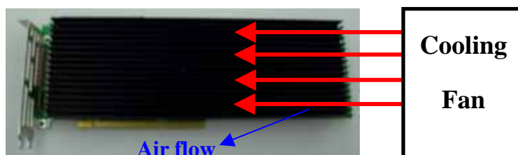
Figure 2. Grape6-BLX64 with cooling fan
