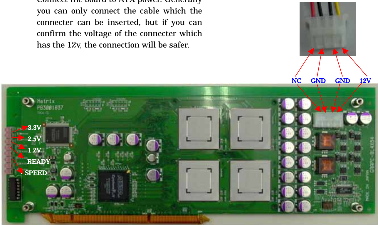
Figure 1. connecting the power cable
