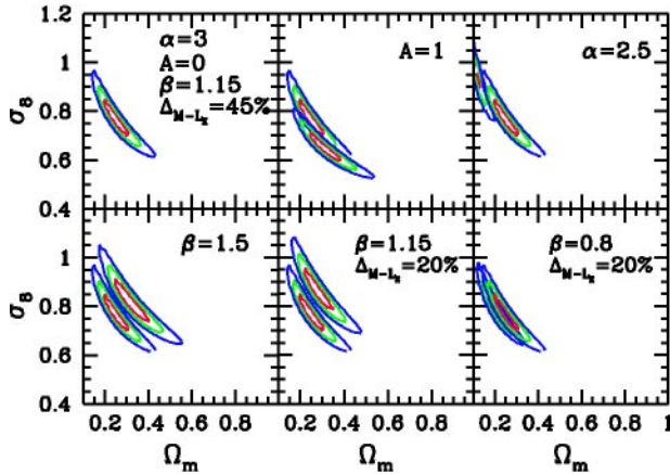
Figure 15 Probability contours in the \sigma_8 - \Omega_m plane from the evolution of the X-ray luminosity distribution of RDCS clusters. The shape of the power spectrum is fixed to \Gamma = 0.2 . Different panels refer to different ways of changing the relation between cluster virial mass, M , and X-ray luminosity, L_X , within theoretical and observational uncertainties (see also Borgani et al. 2001b). The upper left panel shows the analysis corresponding to the choice of a reference parameter set. In each panel, we indicate the parameters that are varied, with the dotted contours always showing the reference analysis.
