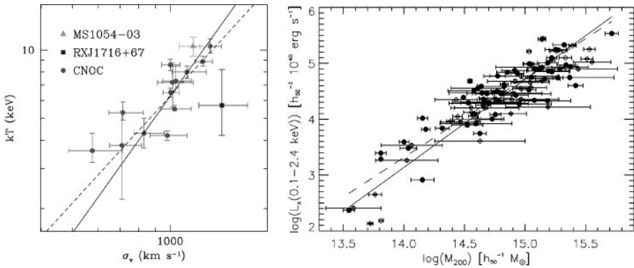
Figure 2 ( Left ) The relation between galaxy velocity dispersion, \sigma_v , and intracluster medium temperature, T , for distant ( z > 0.15 ) galaxy clusters. Velocity dispersions are taken from Carlberg et al. (1997a) for CNOC clusters and from Girardi & Mezzetti (2001) for MS1054-03 and RXJ1716 + 67. Temperatures are taken from Lewis et al. (1999) for CNOC clusters, from Donahue et al. (1998) for MS1054-03, and from Gioia et al. (1999) for RXJ1716 + 67. The solid line shows the relation k_B T = \mu m_p \sigma_v^2 , and the dashed line is the best-fit to the low- z T - \sigma_v relation from Wu et al. (1999). ( Right ) The low- z relation between X-ray luminosity and the mass contained within the radius encompassing an average density 200\rho_c (from Reiprich & Böhringer 2002). The two lines are the best log-log linear fit to the two data sets indicated with filled and open circles.
