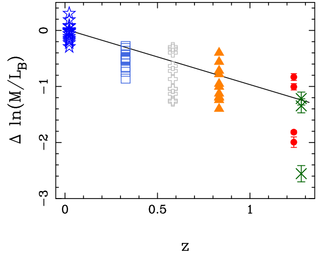
FIG. 3.— Change in M/L_B for early-types as a function of redshift. We use the same symbols as Figure 2 with the addition of light blue open squares for MS 1358+62 (Kelson et al. 2000b, z = 0.328 ), grey open “+” are from MS 2053-04 ( z = 0.583 ) and the filled orange triangles are from MS 1054-03 ( z = 0.832 ), both from Wuyts et al. (2004). The resulting evolution, with respect to the Coma FP, is shown as a line with the form \Delta \ln M/L_B \propto (-0.98 \pm 0.06)z .
