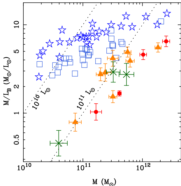
FIG. 5.— M/L_B as a function of mass, using the same symbols as Figure 3 but not including the results for MS 2053-04. The lower redshift trend of higher M/L_B at higher masses appears to be preserved at \bar{z} = 1.25 , even when ignoring the lowest mass galaxy in RDCS 0848+4453. The dotted lines represent L_B = 10^{11} L_\odot and 10^{10} L_\odot . Our z_{850} = 22.5 selection limit corresponds to L_B \approx 10^{10.9} L_\odot for a galaxy with the colors of a Coma elliptical.
