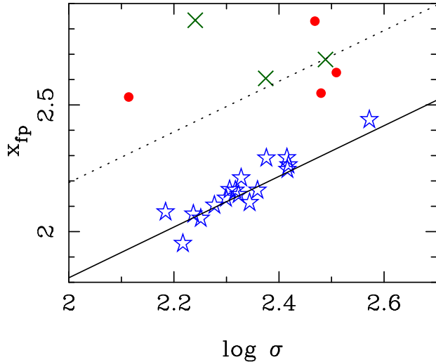
FIG. 2.— A projection of the FP for our sample and Coma. The results for RDCS 1252.9-2927 ( z=1.237 ) are plotted as solid red dots, the green crosses are from RDCS 0848+4453 (van Dokkum & Stanford 2003, z = 1.276 ), and the blue open stars are from Coma (Jorgensen et al. 1996, z = 0.023 ). The y-axis is x_{fp} = 0.83 \log r_e + 0.69 \log l_e , one of the projections of the FP. The solid line is the FP for Coma while the dotted line has the same slope but is shifted \Delta M/L_B = -0.98 for the five massive galaxies at \bar{z} = 1.25 .
