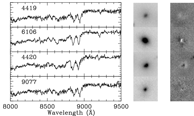
FIG. 1.— Mosaic showing, from left to right, the observed spectra near 4000Å in the rest-frame of the cluster, images and images of the residuals. Each image is 2'' on a side with 0''.05 pixels from the z_{850} ACS data, corresponding to roughly rest-frame Johnson B . The fit results are listed in Table 1. The absolute value of flux in the residuals is \leq 10\% of the flux in the original data. For #4419 and #4420, the residuals have an “S” shape which is interpreted as a sign of interaction (Blakeslee et al. 2003). The residuals for #6106 show an over subtraction in the center, it is likely that the r^{1/4} law is too steep; in this case the best fitting profile is \propto r^{1/3} .
