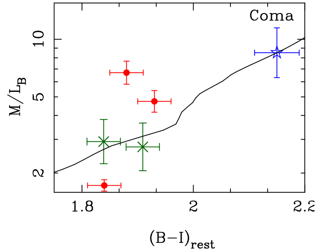
FIG. 4.— M/L_B as a function of the rest-frame Vega B - I color for galaxies with M > 10^{11.5} M_\odot . The average Coma values are represented as a blue star, while the three galaxies from RDCS 1252.9-2927 are solid circles and the two galaxies from RDCS 0848+4453 are green crosses. The line shows the trajectory of a solar metallicity model with an exponentially declining, \tau = 200 Myrs, star-formation rate Bruzual & Charlot (2003) model normalized to the average Coma cluster observations. The highest M/L_B is #4419, the brightest cluster galaxy. The colors of #4419 are significantly bluer than predicted for its observed M/L_B , ruling out the offset being a result of dust or metallicity effects. The lowest mass galaxy in RDCS 0848+4453 is excluded (see text).
