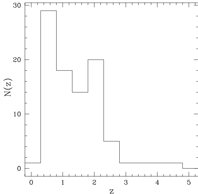
Fig. 3. The photometric redshift distribution of galaxies at R \leq 26.5 in the VLT field.
