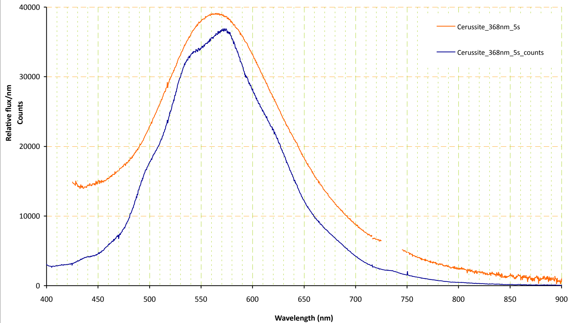
Cerussite, Morocco; 368nm fluorescence Raw counts and flux calibrated
