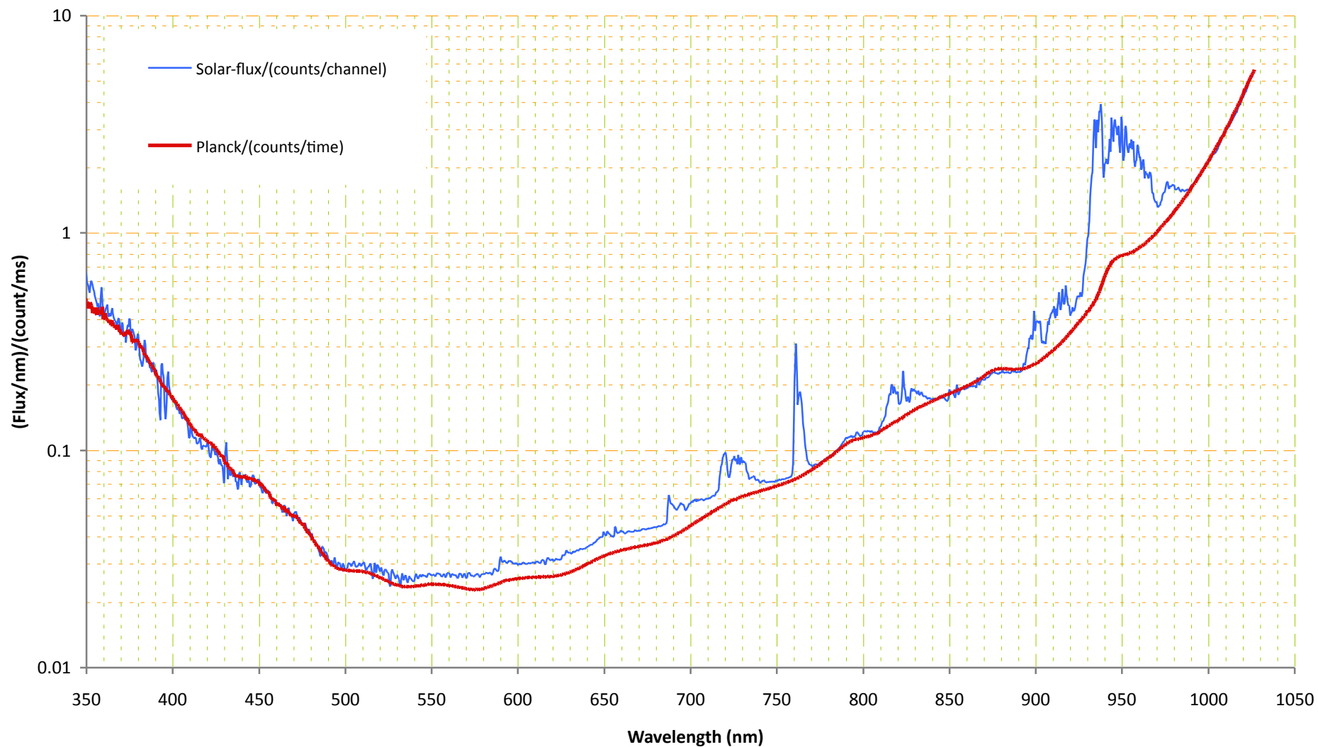
Flux calibration; 23 September 2012, #5 Based on Sun at ZD=51°.5 and IO at 2770K; Ozone=1; Aerosol=3
