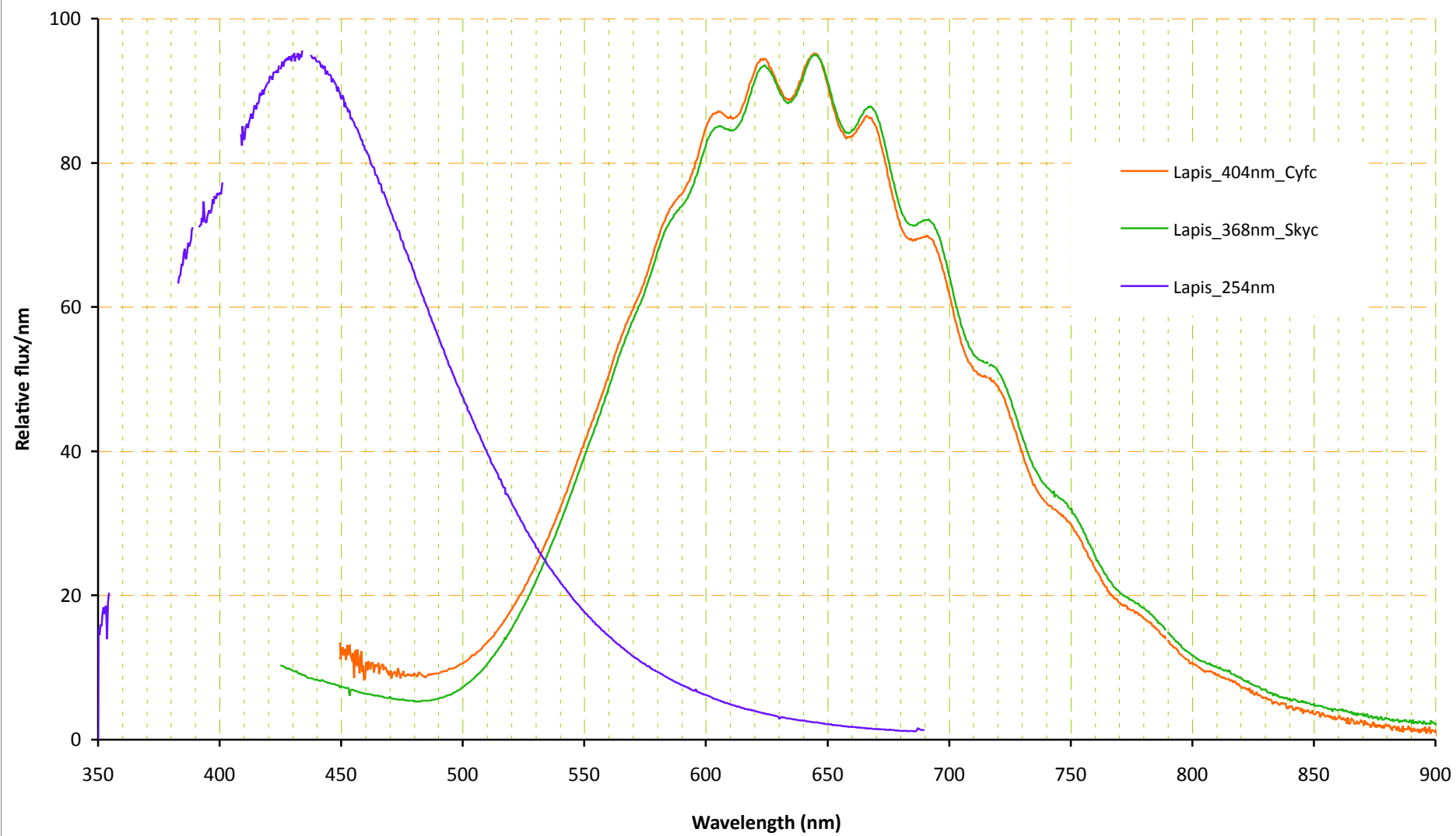
Lapis-lazuli, 254nm (Hg), 368nm (LED) and 404nm (laser) fluorescence
