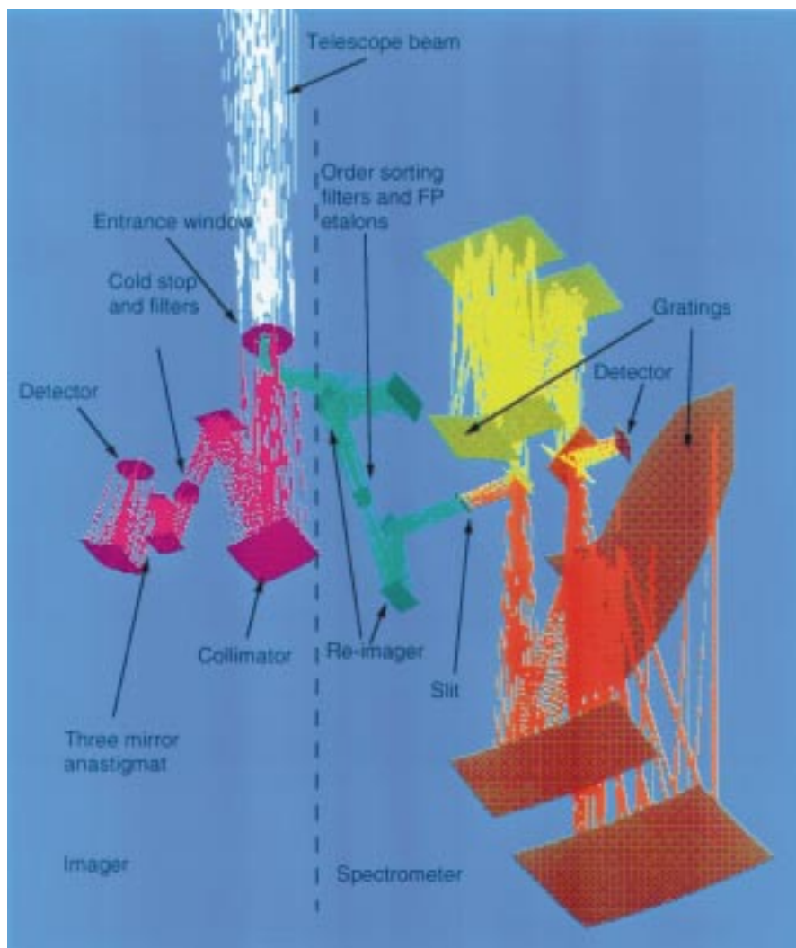
Figure 1: Overview of the optical layout of VISIR. The beam from the telescope is coming from the top. The imager, in pink, is on the left side of the diagram; the spectrometer is on the right side of the diagram. One can see the re-imager unit of the spectrometer in green, the low- and medium-resolution arm in yellow, and the high-resolution arm of the spectrometer in red. The re-imaging unit of the spectrometer was not shown in [1], because we had presented the option where the imager was used as re-imaging unit. This option was no longer viable with the new optical design. The spectrometer re-imaging unit consists of two concave off-axis paraboloids, two folding flats and a cold stop. The order selection filter wheel and the Fabry-Pérot wheel are located immediately behind the cold stop.
