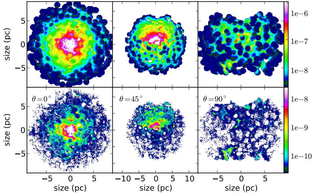
Figure 5. Images at 10\ \mu\text{m} (top) and 0.55\ \mu\text{m} (bottom) of the clumpy AGN torus with N_{\text{clump}} = 1000 and viewing angles (from left to right) of 0^\circ , 45^\circ , and 90^\circ . Color bar gives flux in ( \text{Jy arcsec}^{-2} ). The source with luminosity L = 10^{45}\ \text{erg s}^{-1} is at a distance of 15 Mpc. (A color version of this figure is available in the online journal.)
