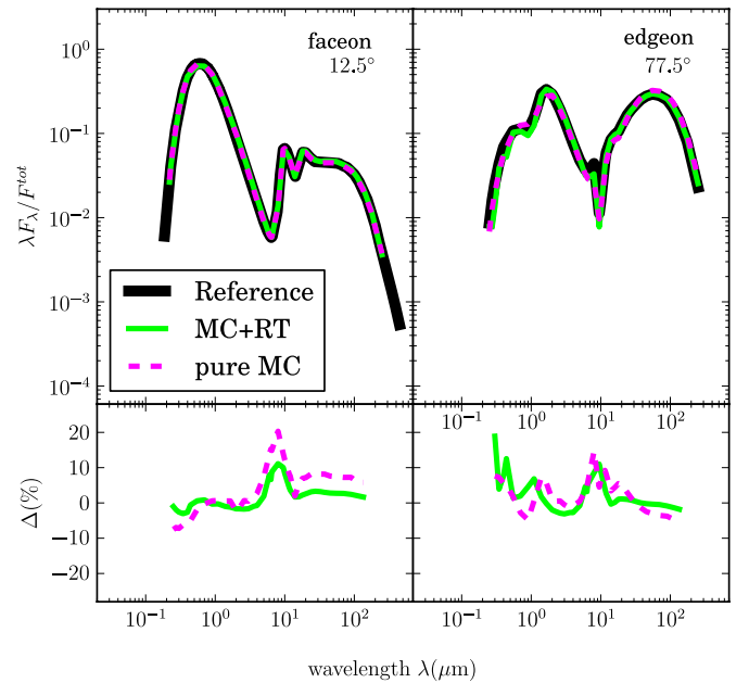
Figure 3. Comparison of SEDs of a dust disk at optical depths along the midplane of \tau_V = 100 , face-on view ( 12.5^\circ ) is shown left and edge-on view ( 77.5^\circ ) right. SEDs are computed with MC and ray tracer (green) or photon counting (dashed). The mean SED of the benchmark results by Pascucci et al. (2004) is in black. Lower panels give the difference between the mean SED of the benchmark and the procedures of this work.
