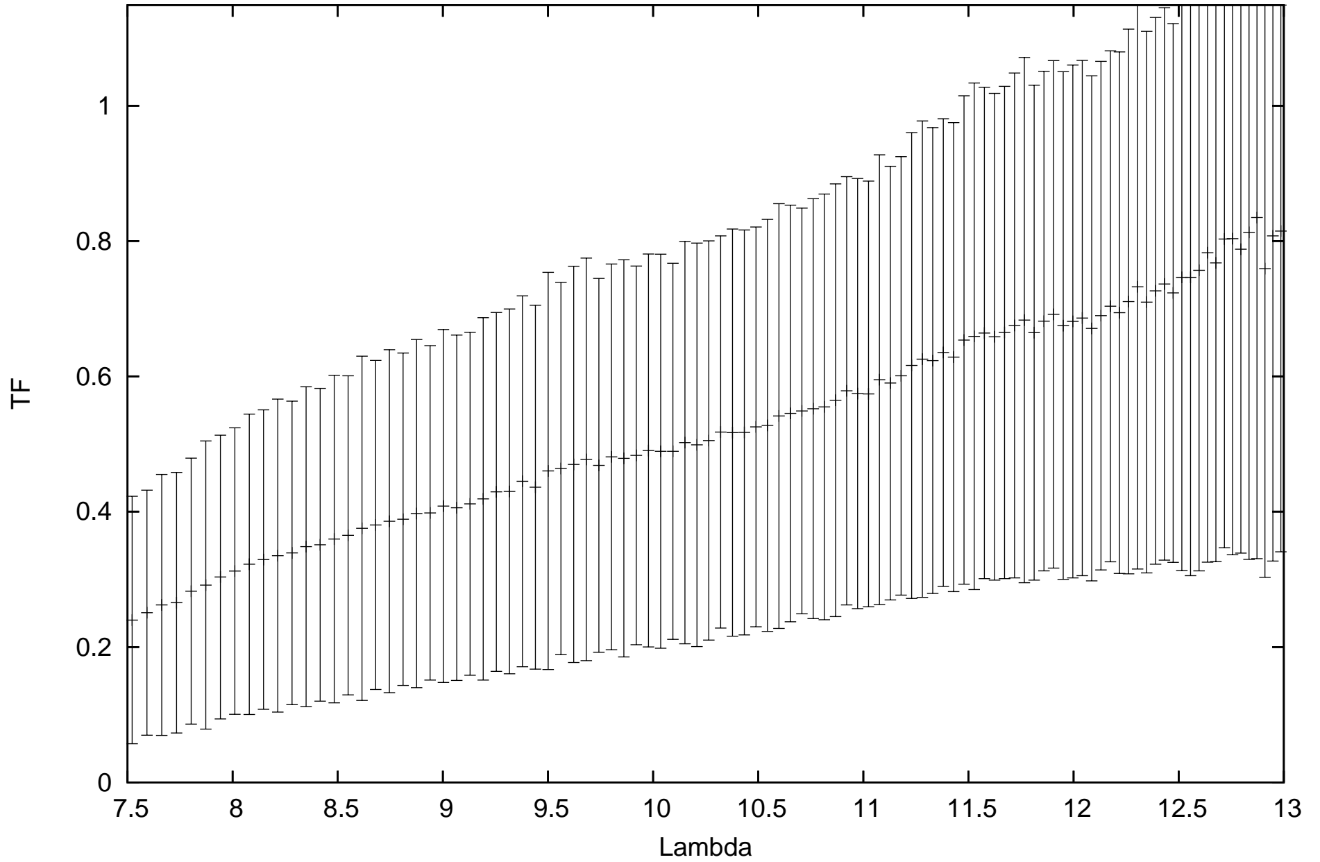
calHD167618_flux-1.82_diam11.66_r.MIDI.2009-08-20T02_39_43.000_HIGHSENS
