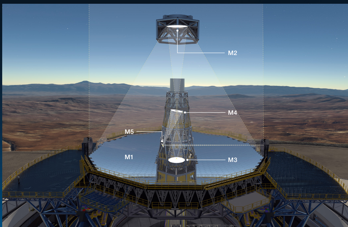
The optical system of the ELT showing the location of the mirrors.
