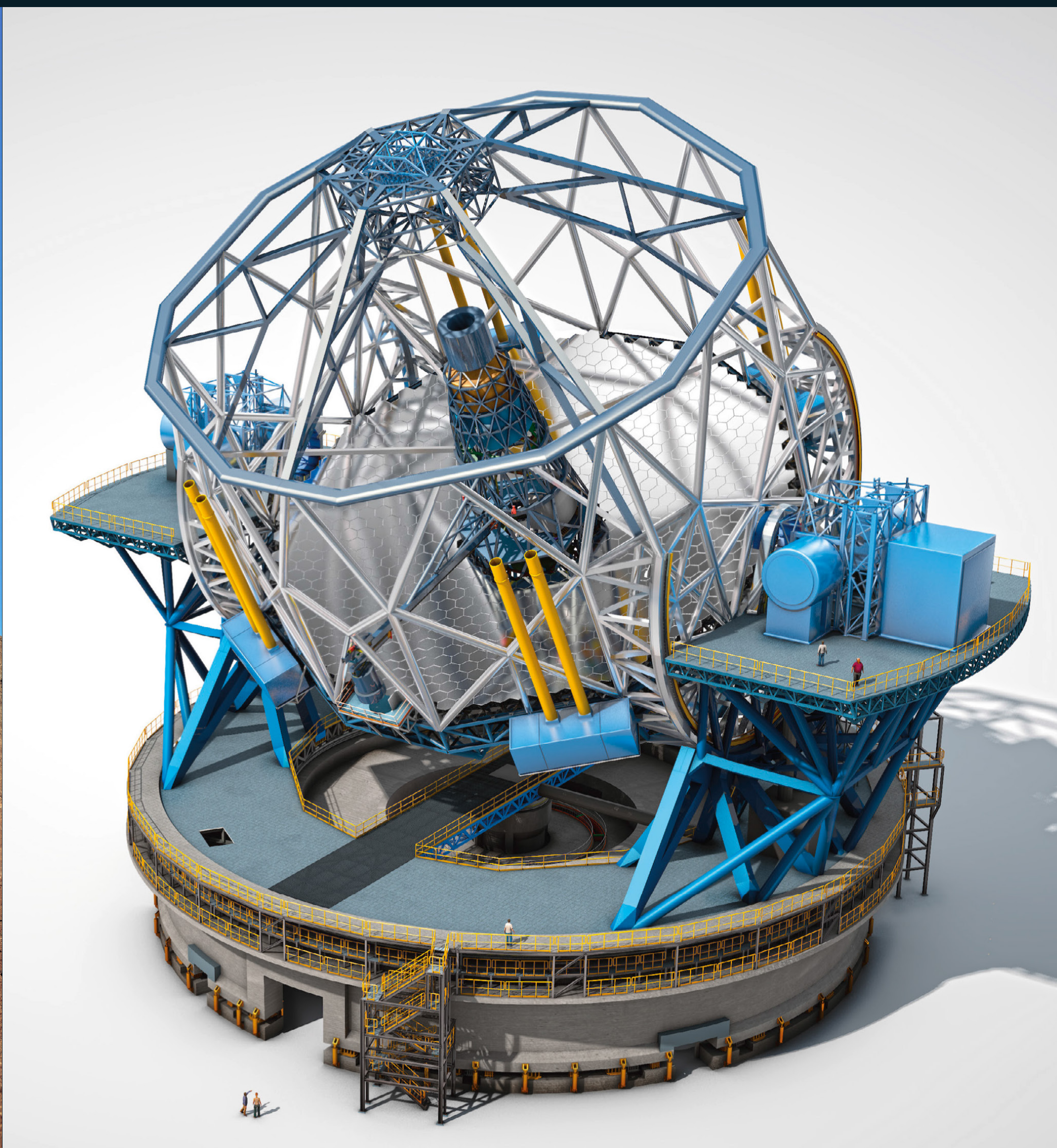
Close-up view of the novel 5-mirror approach of the 39-metre European Extremely Large Telescope (E-ELT) in its enclosure, currently being planned by ESO (artist's impression). Nahansicht des neuartigen Fünf-Spiegel-Systems des European Extremely Large Telescope (E-ELT) in seinem Schutzbau als künstlerische Darstellung so wie es die ESO derzeit plant.
