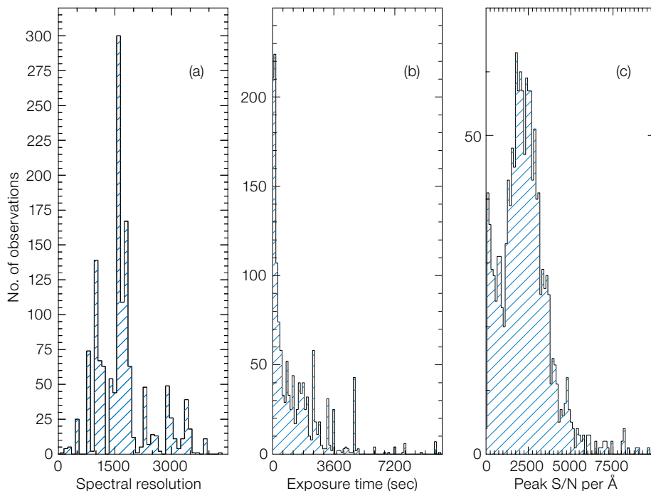
Figure 2. Some statistical data from the analysis of the FORS1 archive of circular spectropolarimetric data. Figure 2a shows the spectral resolution deduced from the analysis of arc lines. The histograms in Figures 2b (shutter time) and 2c (S/N) refer to an observing series (typically composed of eight individual exposures).
