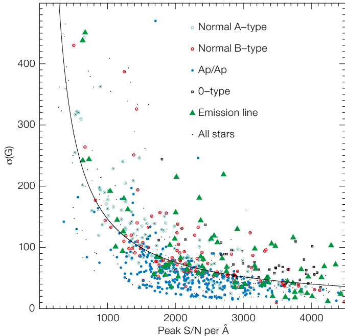
Figure 3. The error bar \sigma(G) from the analysis of all spectral lines as a function of the peak S/N per \text{\AA} for various kinds of stars.
