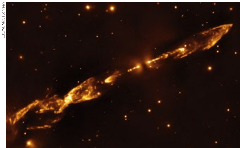
Image in the molecular hydrogen 2.12 \mu\text{m} line of the Herbig-Haro object HH 212 in the Orion B region obtained with the Infrared Spectrometer And Array Camera (ISAAC). The spectacular collimated bipolar outflow from the central young star shocks against the local cloud material, producing a typical emission spectrum strong in molecular hydrogen, other more complex molecules and ionised gas.
