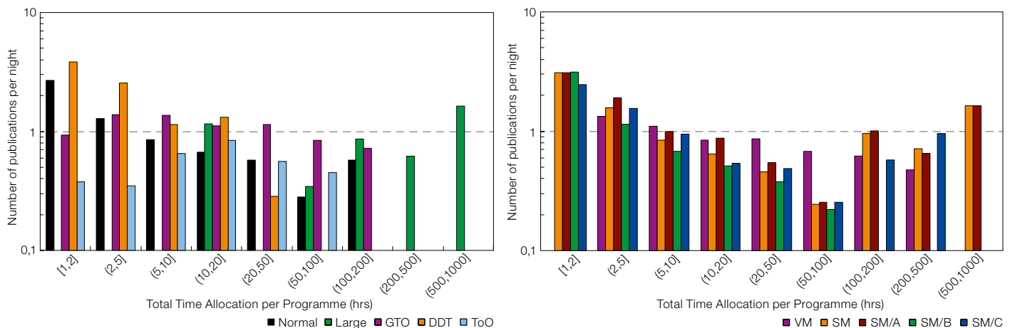
Figure 2. The dependence of productivity, by programme type (left panel) and observing mode and SM rank classes (right panel), in terms of publications per night is shown for the total time allocation per programme.
