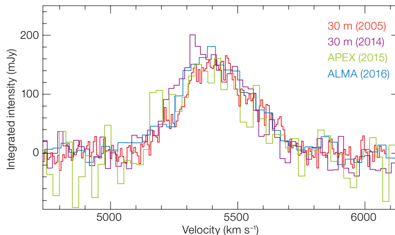
Figure 5. The H 2 O 183.3 GHz line as observed with the IRAM 30-metre telescope in 2005 (Cernicharo et al., 2005) and 2014, with SEPIA on APEX in 2015 (Galamez et al., 2016) and with ALMA in 2016 (König et al., 2017), displaying the relative constancy of the line profile. From König et al. (2017).
