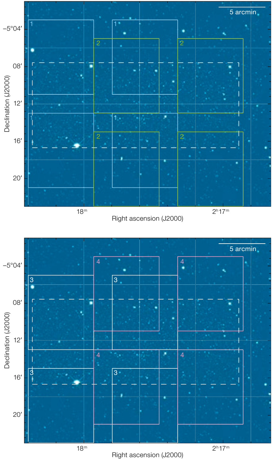
Figure 1. Illustration of how the four VANDELS VIMOS pointings are organised within the UDS survey field. The rectangle indicated by the dashed white line shows the region covered by deep H -band HST imaging from the CANDELS survey. The four VIMOS pointings (labelled 1–4), each with four quadrants, are located to ensure that 100% of the HST
