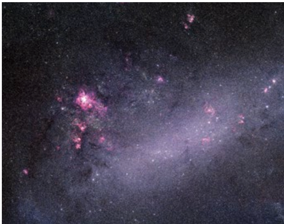
A wide-field image (about 4 degrees in extent) of the Large Magellanic Cloud and 30 Doradus taken by the ESO 1-metre Schmidt telescope in 1986, before the appearance of SN 1987A.
