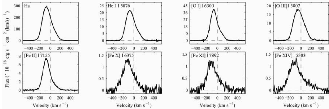
Figure 3: Intermediate-velocity component from the cooling, shocked material from the inner ring, showing a range of ionization stages, including highly ionized coronal lines from gas at \sim 2 \times 10^6 K (from Gröningsson et al. 2006)
