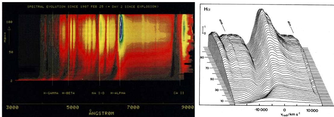
Figure 2: Spectral evolution of SN 1987A as observed with the Bochum telescope (Hanuschik and Thimm 1990). Important lines are marked at the bottom. The evolution covers the first 120 days and the redshifting of all lines is easily visible. The Bochum event is shown in the right panel displaying the H \alpha evolution as the blueshifted excess.
