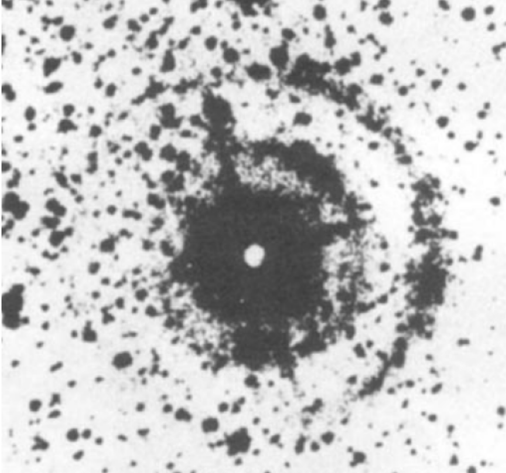
Figure 4: Expanding light echoes around SN 1987A (NTT image reproduced in Arnett et al. 1989)
