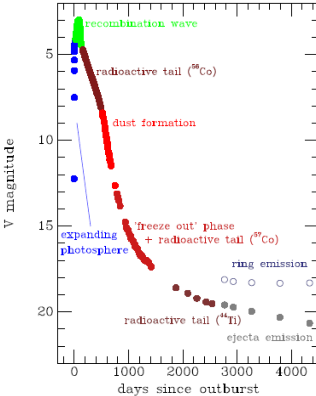
Figure 1: Light curve of SN 1987A over the first 12 years. The figure marks some of the most important events in the history of the supernova (from Leibundgut & Suntzeff 2003).
