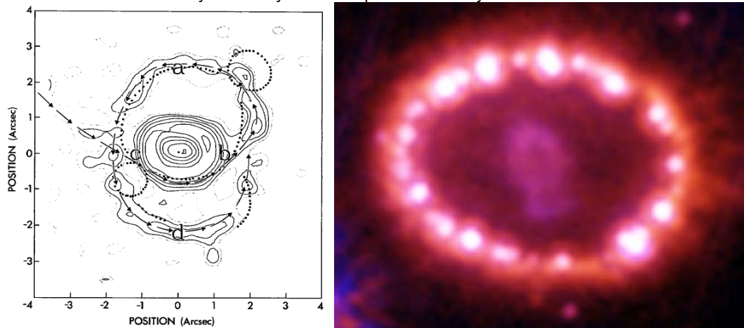
Figure 3: NTT image of the circumstellar environment of SN 1987A (left; Wampler et al. 1990) and the ring in 2003 as observed by HST
