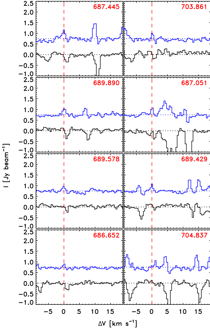
Fig. 3.— Zoom-in on the glycolaldehyde transitions predicted to be most optically thick at 690 GHz toward the IRAS16293B continuum peak ( black ) and toward a position offset by one synthesized beam from the continuum peak ( blue ; shifted by 0.75 \text{ Jy beam}^{-1} in the Y-axis direction). As in Fig. 2 the velocities on the X-axis is given relative to the systemic velocity.
