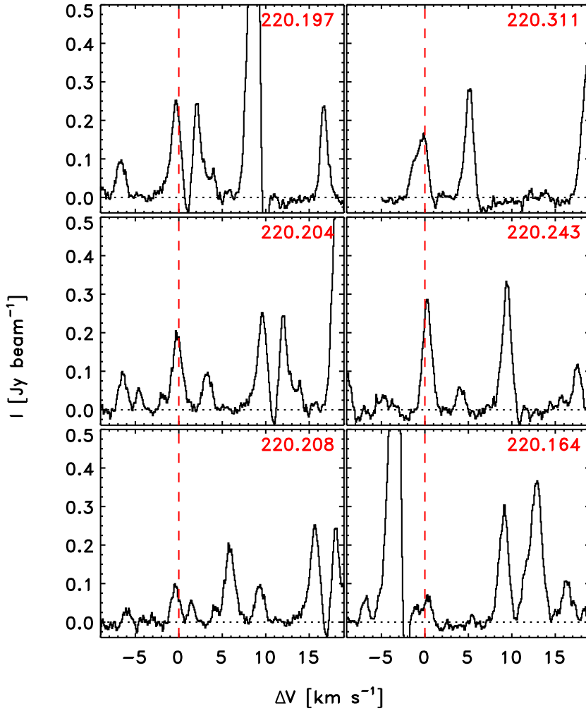
Fig. 2.— Zoom-in on the glycolaldehyde transitions detected at 220 GHz. The velocities on the X-axis is given relative to the systemic velocity of 2.7 km s ^{-1} .
