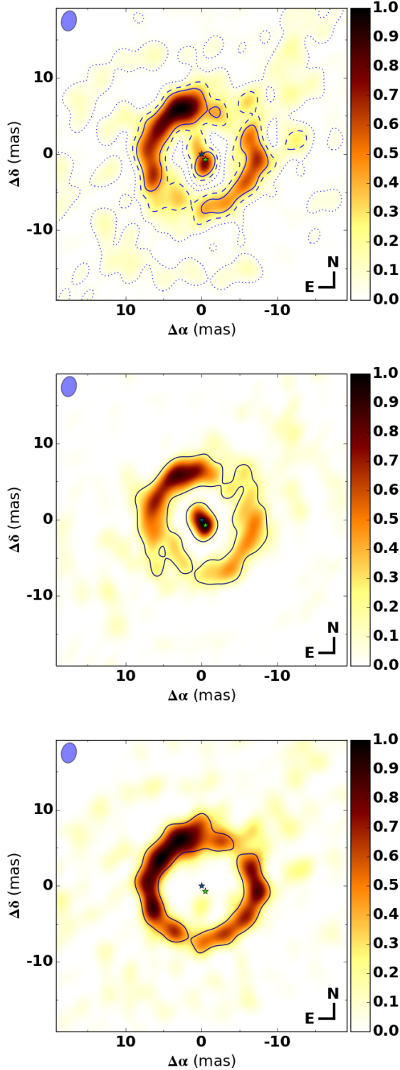
Fig. 4. The reconstructed images. Upper panel: single-star-subtracted reconstruction of the original data. Middle panel: single-star-subtracted construction of the synthetic data set made with the best-fit parametric model. Lower panel: binary-subtracted reconstruction of the original data. The horizontal and vertical axes contain right ascension and declination coordinates in units of milli-arcseconds, respectively (the north and east directions are indicated in the lower right corner). The blue ellipse shows the beamsizes. The full, dashed and dotted lines delineate pixels that have fluxes above 5\sigma , 3\sigma and 1\sigma , respectively. For clarity only the 5\sigma contours are shown in the lower panels. The blue and green star symbols indicate the positions of the two stars as determined from the best-fit parametric model (the actual flux of the primary is subtracted from the image). The color indicates normalized flux, scaled to the highest pixel value in the image.
