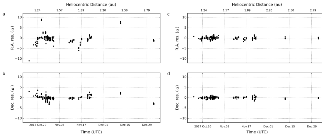
Figure 2. Astrometric residuals of ‘Oumuamua observations. a, b: normalized right ascension and declination residuals against a gravity-only solution. c, d: normalized right ascension and declination residuals against a solution that includes a non-gravitational radial acceleration A_1 r^{-2} . As each residual is normalized to its standard deviation, each data point has a 1 s.d. error bar equal to 1 on this scale.
