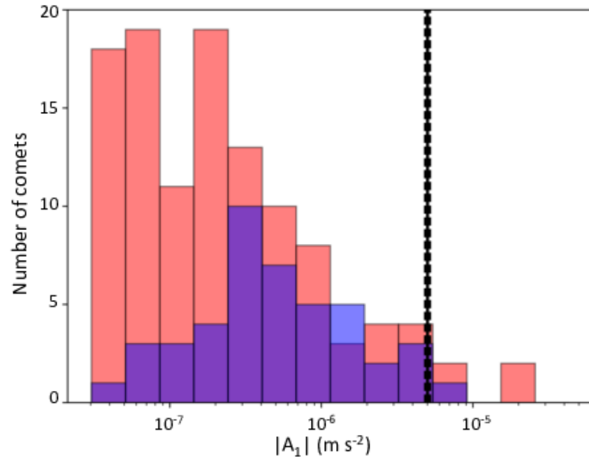
Extended Data Figure 1. Non-gravitational accelerations of Solar System comets and 'Oumuamua. Measured non-gravitational radial accelerations A_1 for short-period (red) and long-period (blue) comets from the JPL Small Body Database. The solid vertical black line indicates the A_1 value for 'Oumuamua, which falls within the range observed for Solar System comets, while the dashed vertical black lines mark the corresponding 1\sigma uncertainty.
