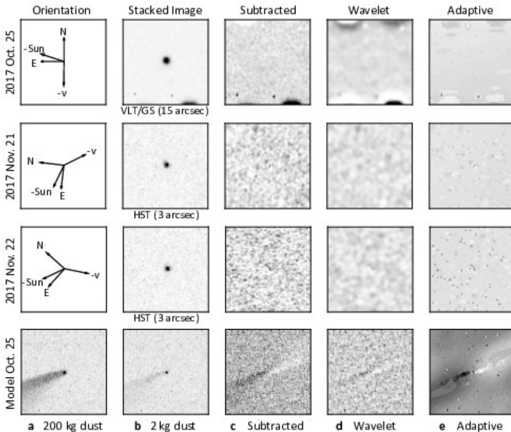
Figure 1. Deep stacked images for dust detection. For each date we show the image orientation (-Sun=anti-solar, -v=anti-motion direction), the stacked image, a self-subtracted image (see Methods), and the image after application of a wavelet and adaptive filter to enhance low surface brightness features. No dust is visible. A model image with an artificial cometary feature matching the October geometry demonstrates the sensitivity of the image enhancement. The panels show (a) a very strong dust feature; (b) the same feature scaled to 2 kg of dust in the PSF region (twice the observed 'Oumuamua limit), (c) (d) (e) processed in the same manner as the real data.
