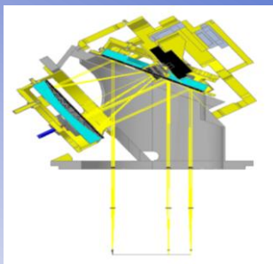
Pupil Reimager of NIRVANA
