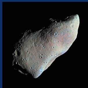
Asteroid Gaspra (NASA Galileo 1991)
