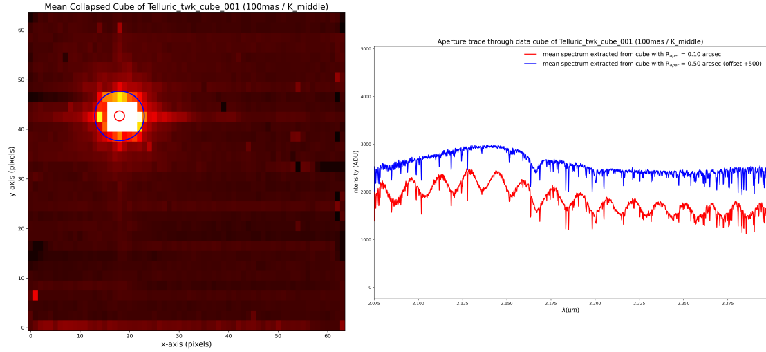
Figure 3: an example of extracted spectrum “wiggles” in an under-sampled ERIS/SPIFFIER standard star. Being under-sampled, the majority of the stand star’s flux falls into a single rectangular spaxel. When extracting through the data cube over an aperture close to this single pixel (the red aperture in the collapsed cube shown on the left), the undulating spectrum becomes apparent (red trace: right-hand panel). When extracted over a reasonable aperture (blue aperture), the under-sampled wiggles average out (blue trace offset by 500 ADU).
