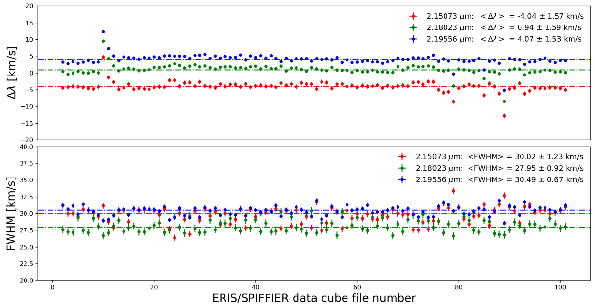
Figure 1: the wavelength shift (top panel) and FWHM (bottom panel) for three [OH] lines, as measured in a sample of 100 ERIS/SPIFFIER data cubes in K middle /100mas. These observations were made in a wide variety of pointings (i.e. the full range of accessible altitudes and instrument rotator angles).
