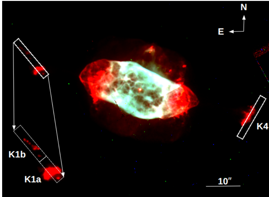
Figure 1: RGB image of NGC 7009 (R: [N II] \lambda 6584 , G: Ha, B: [O II] \lambda 5007 ) from HST data. The white rectangles illustrate the position of the X-Shooter slits centered on the East and WEST LISs. The zoomed-in image of the eastern K1 LIS shows the individual regions that we chose to extract the spectra (K1a, K1b). For K4 the extracted regions is the one in which we can see [NII] emission.
