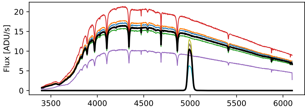
OIII+50 response curve (0.3" and 0.5" slits)
