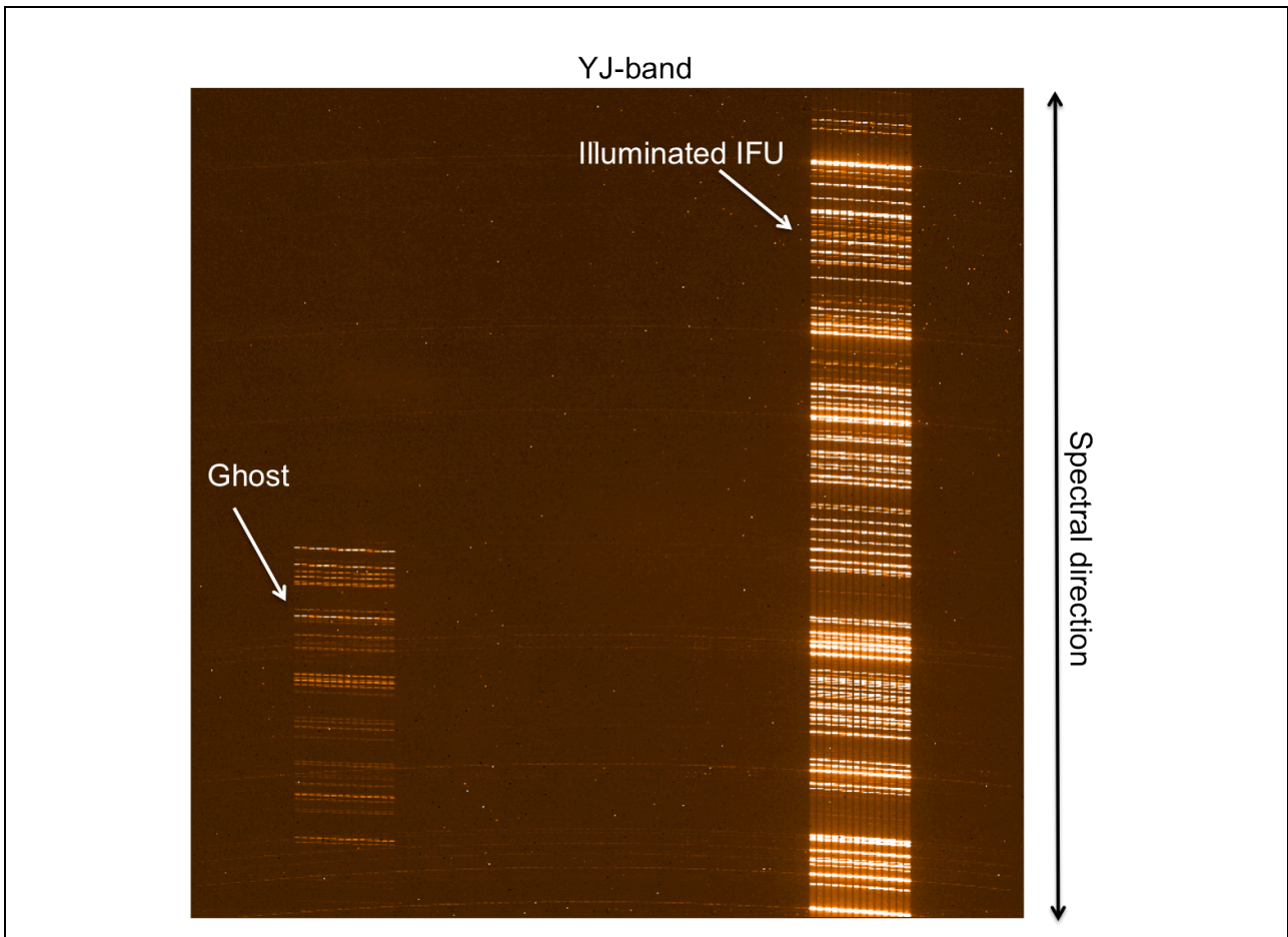
Figure 17. Image in the YJ-band, with one single IFU illuminated with a Argon+Neon calibration lamp (on the right). The ghost is visible on the left side of the array. The colour scale has been enhanced to show the ghost, since the level of the ghost is less than 1% for all bands.
