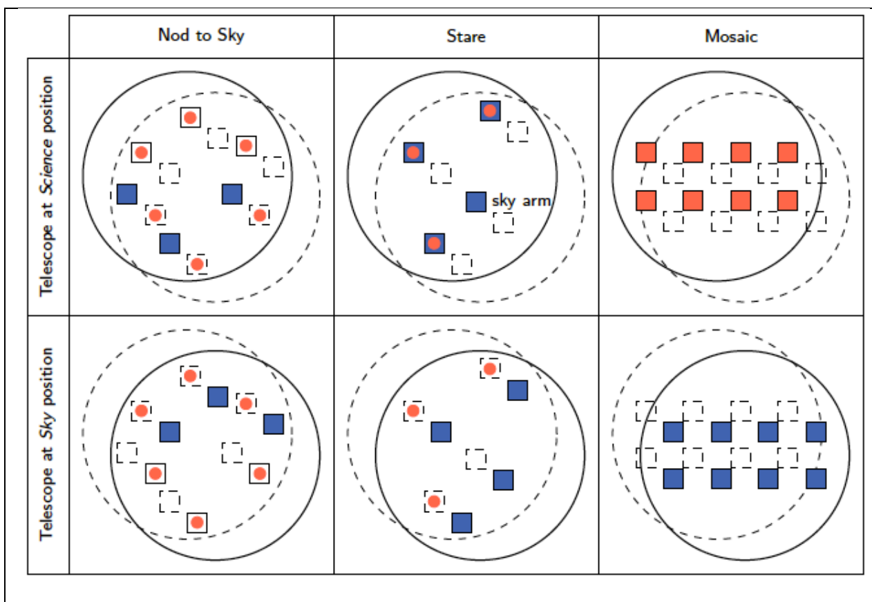
Figure 10 Schematics of the three observation modes configurable by KARMA: Nod to Sky, Stare and Mosaic. Depending on the current telescope position, an arm is either allocated to a science target or to sky background. The offsets between Science and Sky position are performed by the telescope alone while the pick-off arms remain fixed at their positions in the focal plane. (Only a few IFUs are depicted). Not drawn to scale.
