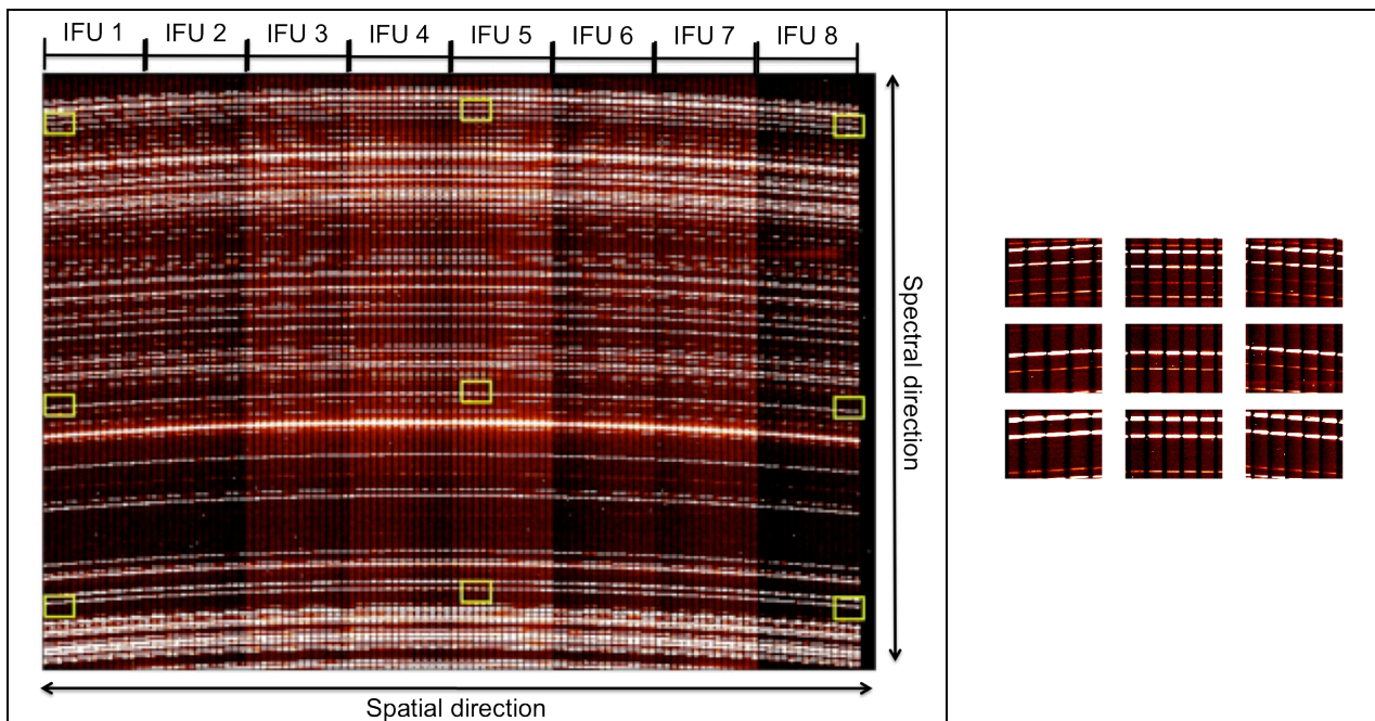
Figure 8. Left: One full detector showing the light from the arc calibration lamp (argon + neon) in the H-band. The location of the edges of the 8 IFU imaged onto the detector is shown at the top of the image. The yellow squares on the image mark 9 positions for which a zoom-in is provided in the right panel.
