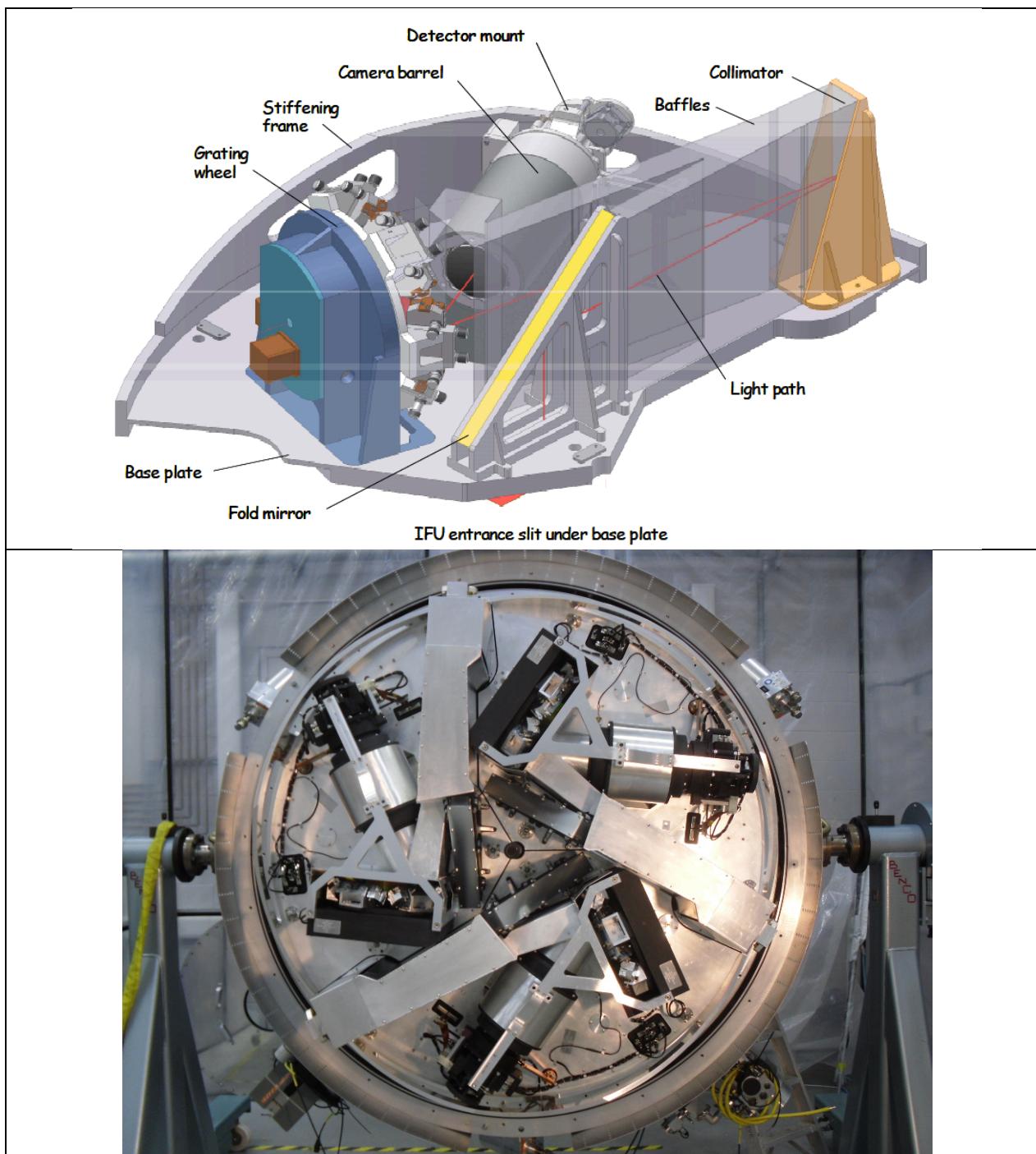
Figure 5. Top: Perspective view of a single KMOS spectrograph module. Bottom: the three spectrographs mounted in the KMOS cryostat.
