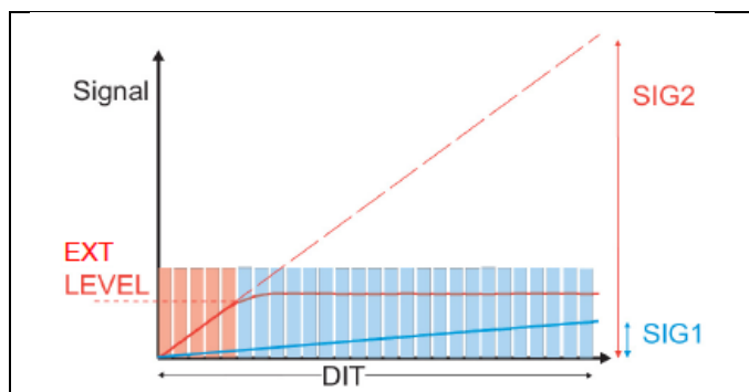
Figure 6. Extrapolation threshold for nondestructive sampling and extrapolation of detector signal for high flux levels. For pixels with high flux (red) only readout values below EXTLEVEL (orange rectangles) are taken into account in the calculation of the slope and values written in the FITS files are extrapolated to the full DIT (SIG2). For low flux pixels (blue) all nondestructive readouts are used (light blue rectangles). This is a modified figure from Finger et al. (2008). A document explaining in detail this readout mode, and its different regimes with their consequences, is available at:
