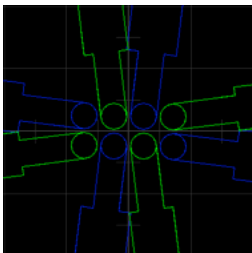
Figure 21 Positions of arms during observations with template KMOS_spec_obs_mapping8.
