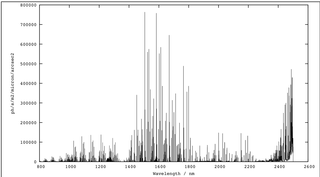
Figure 12. Sky emission as a function of wavelength.
