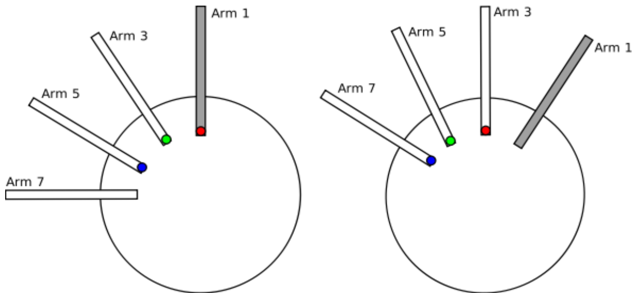
Figure 23 Idea behind rotator optimization: Let Arm 1 be locked e.g. after a hardware failure. Left: In the original configuration given by the KARMA set up file the red target cannot be observed. Right: After rotating the instrument and recalculating the mapping between targets and arms all targets are observable. An optimization like this might be of special interest if the red target has higher priority than the others.
