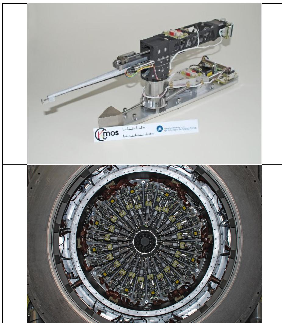
Figure 3. Top: one of the pick-off arms; Bottom: the full 24 pick-off arms in the front end of the KMOS cryostat.
