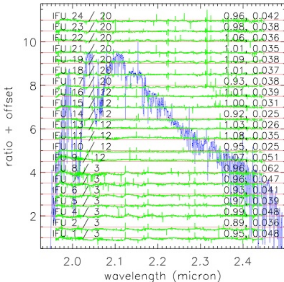
Figure 16. Comparison between the measurements of the 3-arm standard star template and all 24-arms sciencepattern standard star template. In the 3-arm standard star the IFU used are number 3,12 and 20 (one per each spectrograph). The blue curve in the background shows the extracted spectrum for a standard star in the K-band. The overplotted green curves are the ratio (in arbitrary scales and offsetted) between the spectra in each IFU respect to those taken in the just the 3 reference arms (3,12,20) taken via the 3-arm standard star template, as labelled on the left hand side. For each IFU on the right it is indicated the mean ratio and the standard deviation.
