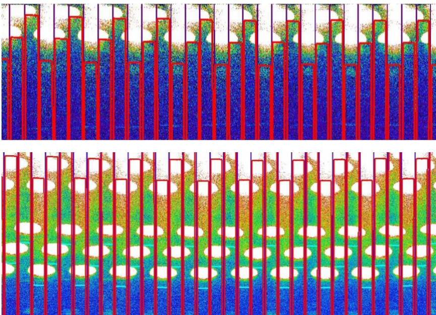
Figure 19: Second order effect in nominal (top panel) and extended (bottom panel) modes, shown here for a bright exposure with arc lines. The red boxes mark the slice limits up to 930 nm. The impact of second order is visible as the white ellipses illuminating the top of the detector. The nominal instrument mode is not affected by contamination, but it is more significant in the extended instrument mode.
