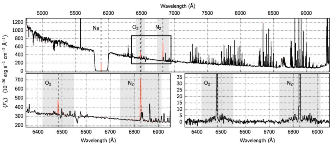
Figure 23 Sky spectrum seen by MUSE with 4LGSF on in WFM-AO mode.
