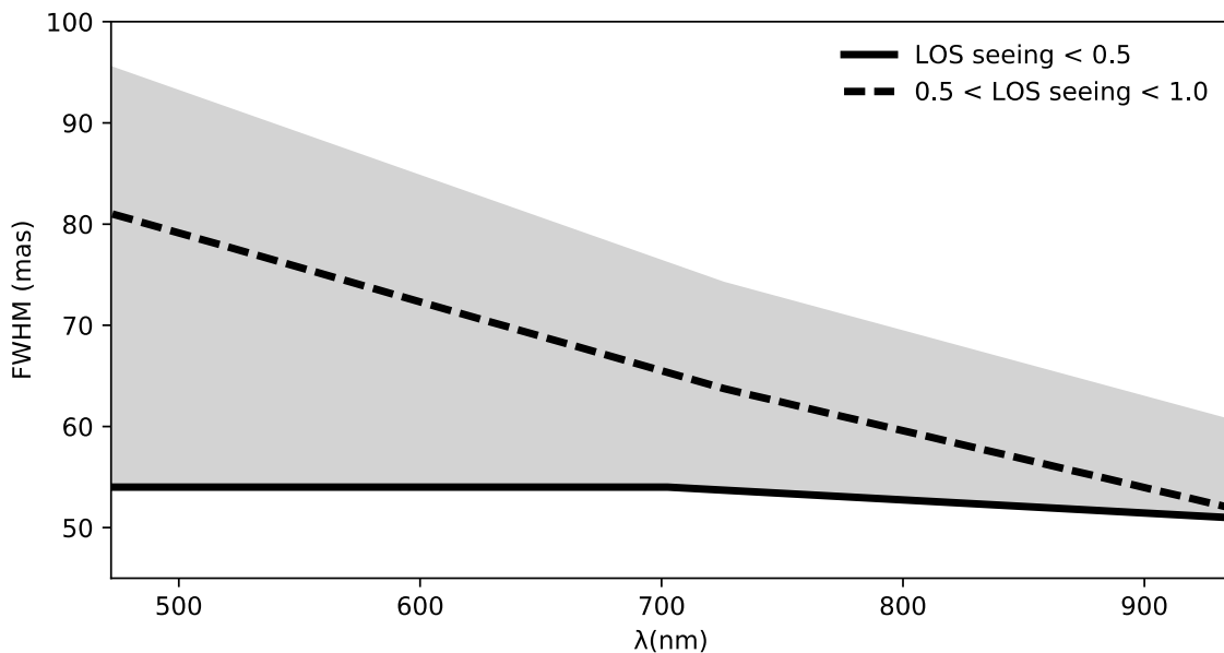
Figure 20: FWHM of the MUSE NFM PSF peak as a function of wavelength. The solid line represents the very best performance in the best seeing conditions with a seeing (at 500 nm) along the line of sight (LOS) <0.5". The dashed line shows the median performance for a seeing along the line of sight between 0.5" and 1.0". The grey area shows the observed variation of the FWHM recorded during the commissioning runs, depending on details of the atmospheric turbulence profile.
