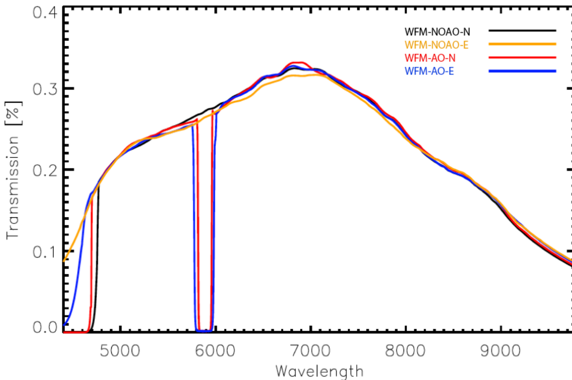
Figure 15: End-to-end MUSE+VLT/UT4 throughput in WFM, as derived from spectroscopic standard observations.
