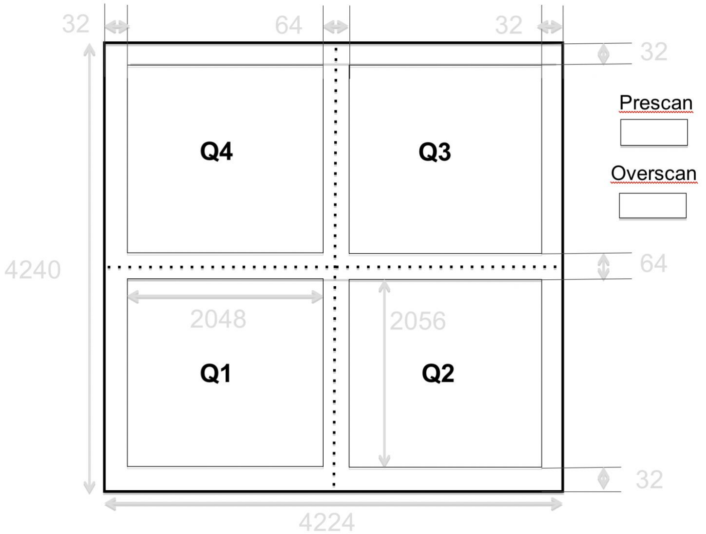
Figure 9: Overview of the pixel map of one of the detectors, showing the 4 quadrants and the pre-scan / over-scan regions. All scales are given in pixels.
