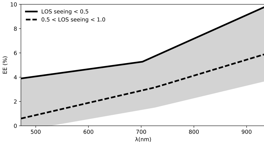
Figure 21: Ensquared Energy (EE) in a 25mas (one spaxel) box as a function of wavelength. As in, Figure 20, the continuous line shows the best performance for a LOS seeing <0.5". The dashed line shows the median performance and the grey area indicates the range observed during the commissioning runs for a LOS seeing between 0.5 and 1 arcsec.
