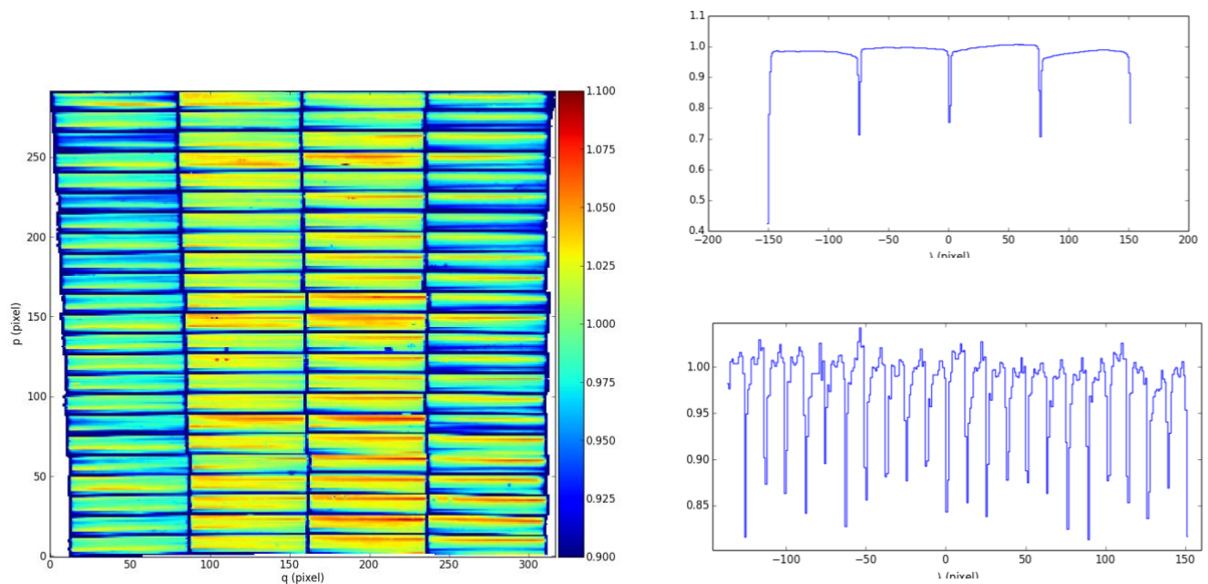
Figure 18: (left) normalized reconstructed image of the continuum flat-field in WFM. (right) horizontal (top) and vertical (bottom) cuts through the normalized image showing the horizontal and vertical variations in illumination.
