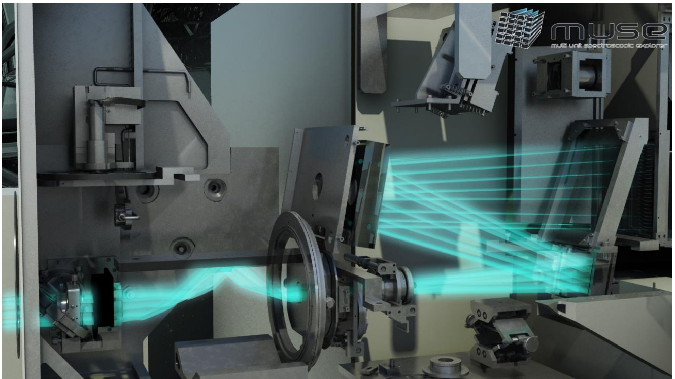
Figure 3 MUSE fore-optics schematics in NFM configuration
