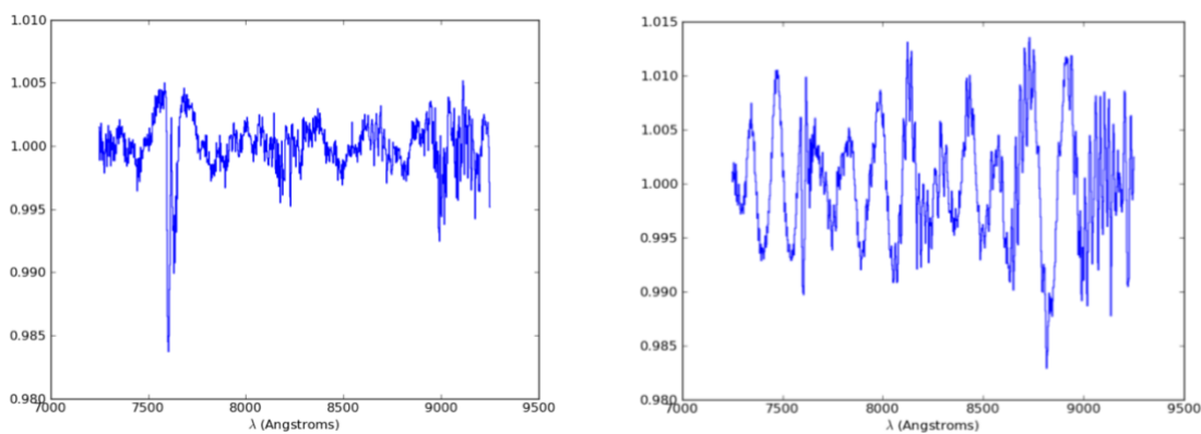
Figure 22: Fringing measured in the red, measured on normalised flat-field frames. (left) WFM, (right) NFM.
