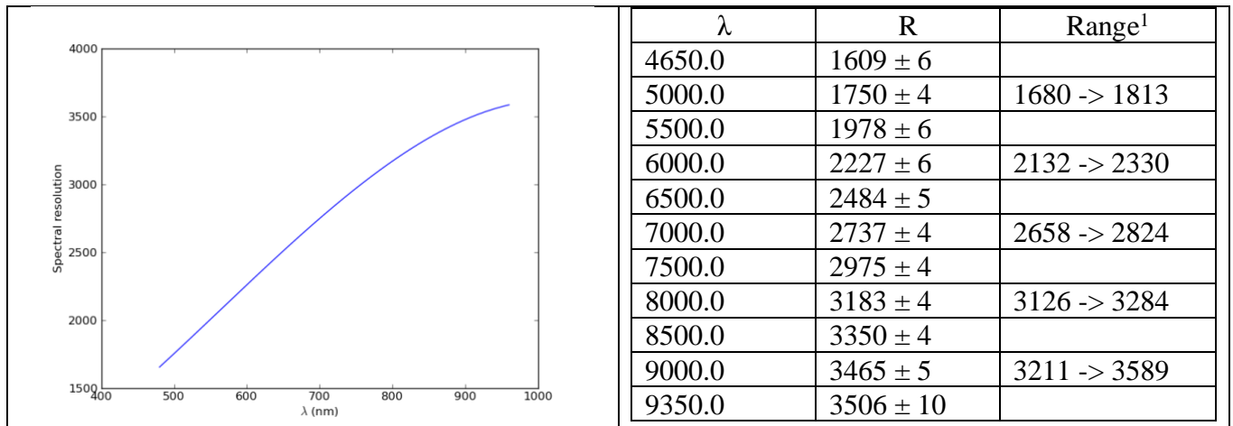
Figure 17: Spectral resolution, R = \lambda/\Delta\lambda , as a function of wavelength, as measured in the lab using calibration lamps. 1 Range over channels. From Technical Note ESO-318117.
